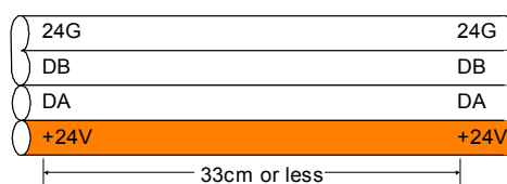
Figure B.5 – Flat cable polarity marking
