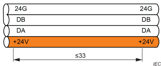
Figure B.5 – Flat cable polarity marking
