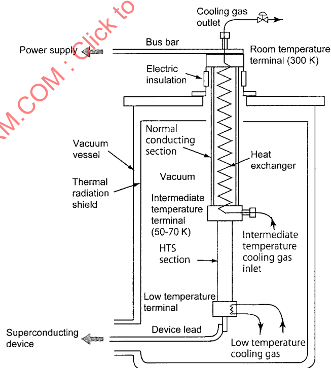
Figure B.3 – Schematic diagram of current leads composed of forced flow cooled normal conducting section and HTS section in vacuum environment
