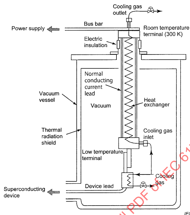
Figure B.2 – Schematic diagram of forced flow cooled normal conducting current leads
