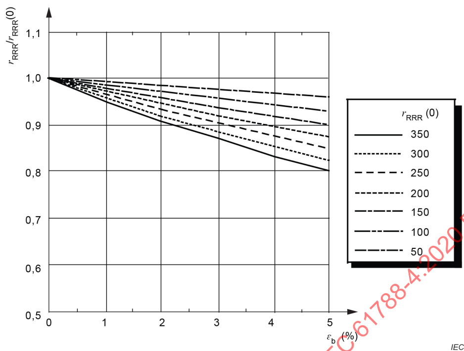
Figure A.4 – Bending strain dependency of normalized RRR value for round Cu wires
