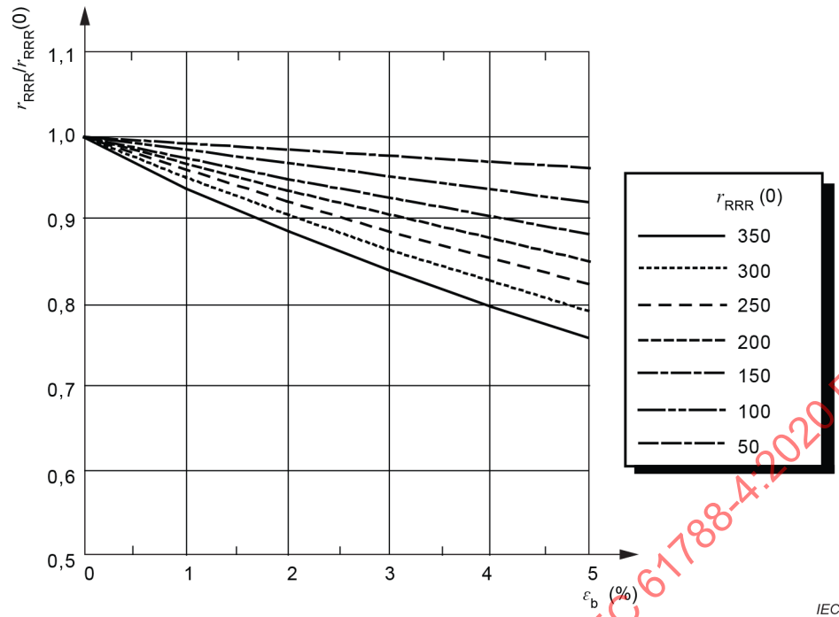
Figure A.6 – Bending strain dependency of normalized RRR value for rectangular Cu wires
