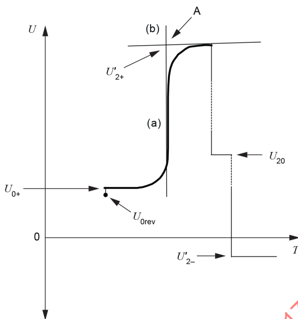
Figure A.1 – Definition of voltages
