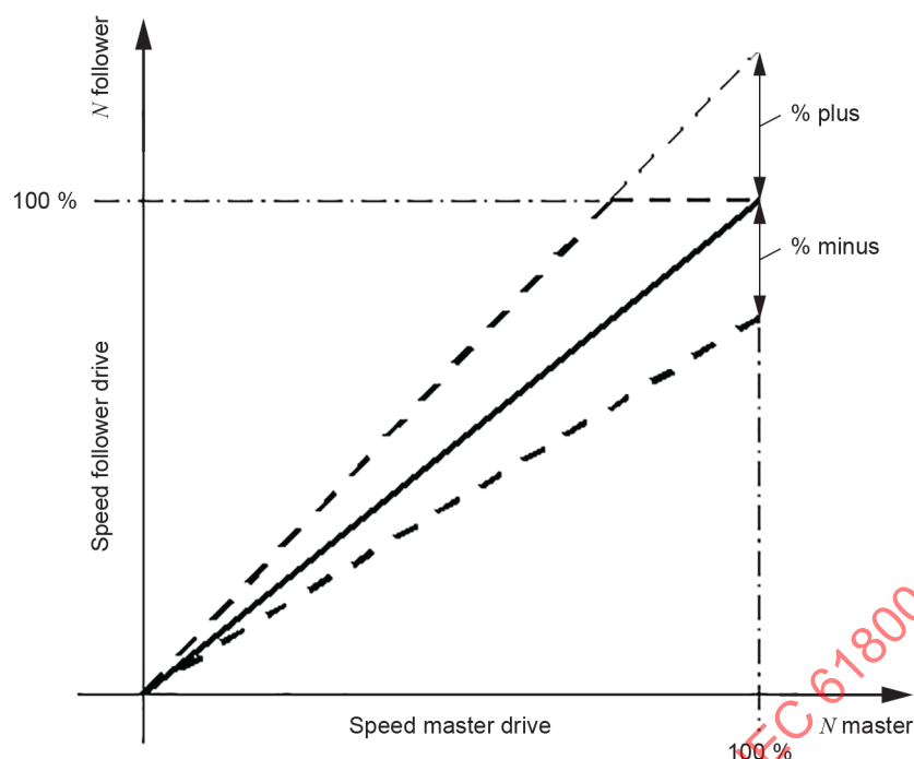
Figure D.3 – Master/follower drive system
