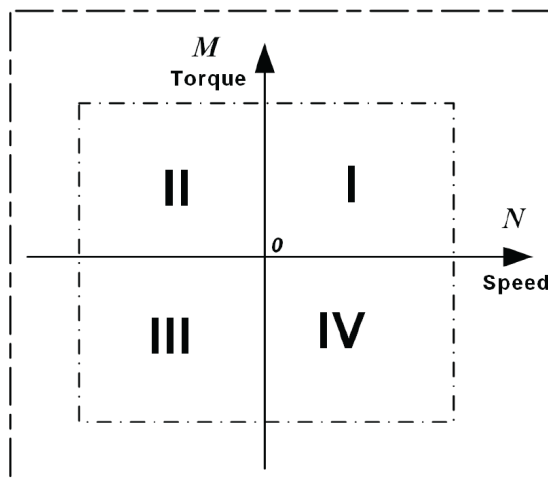
Figure 4 – Operating quadrants
