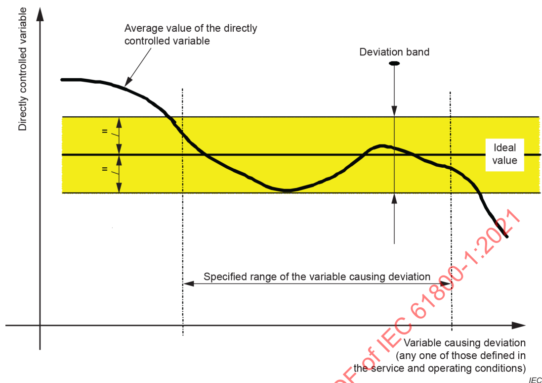
Figure 10 – Deviation band
