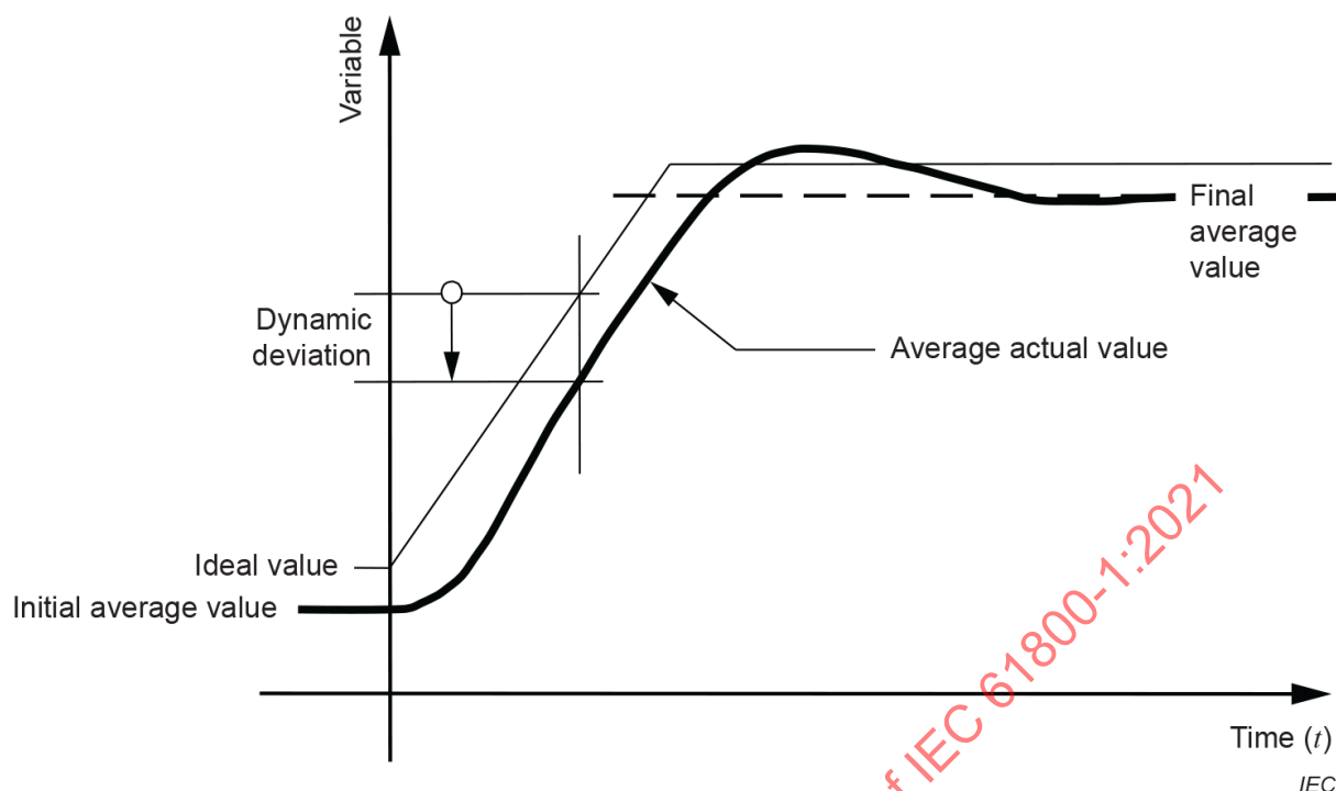
Figure 13 – Time response following a reference change at specified rate
