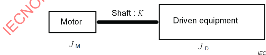
Figure D.6 – Mechanical diagram
