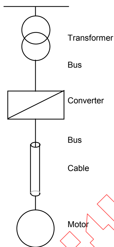
Figure E.3 – Example of drive
