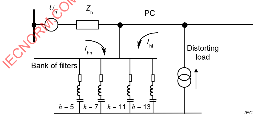
Figure C.4 – Example of passive filter battery
