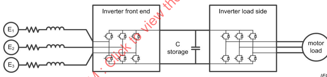
Figure C.8 – Front-End inverter system
