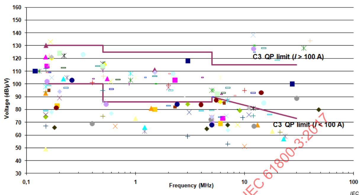
Figure D.1 – Conducted emission of various unfiltered PDS
