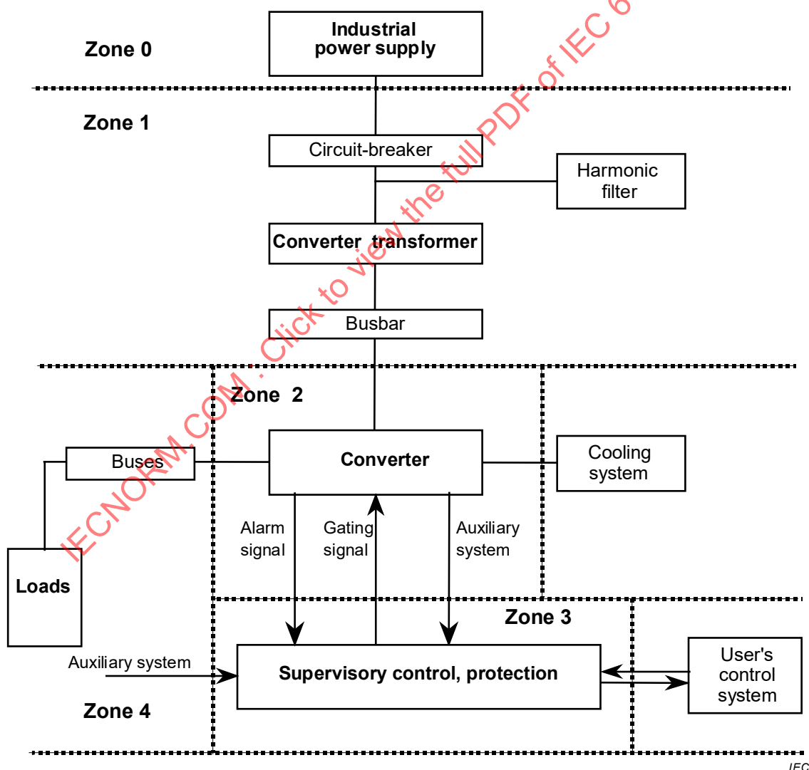
Figure E.2 – Zone concept
