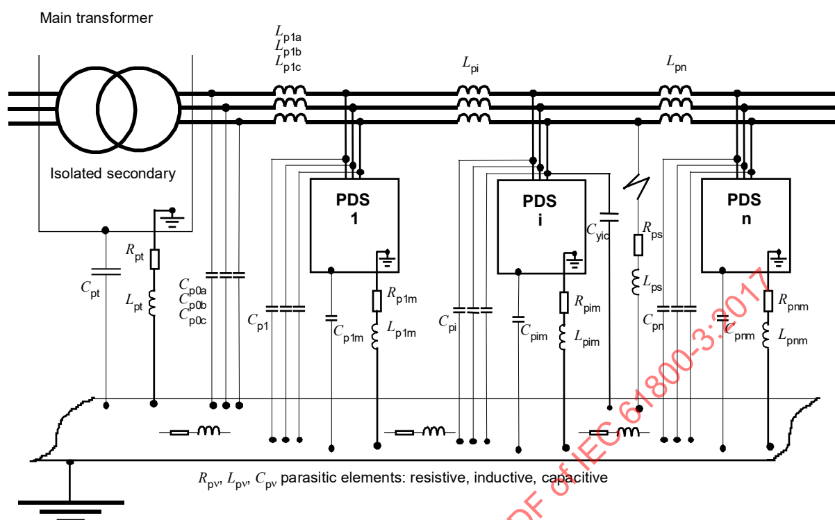
Figure D.3 – Safety and filtering
