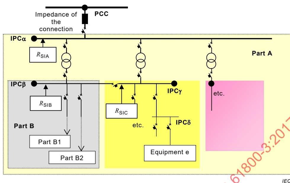
Figure B.2 – PCC, IPC, installation current ratio and R_{Sl}
