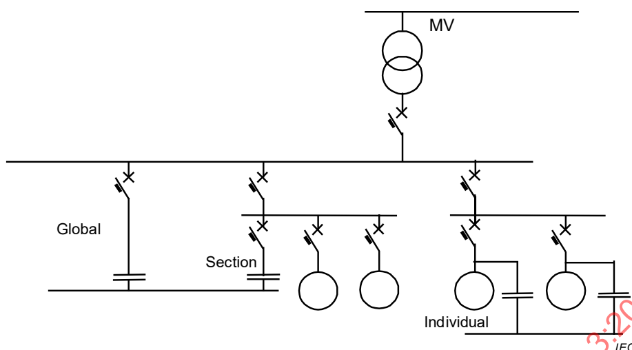
Figure C.1 – Reactive power compensation
