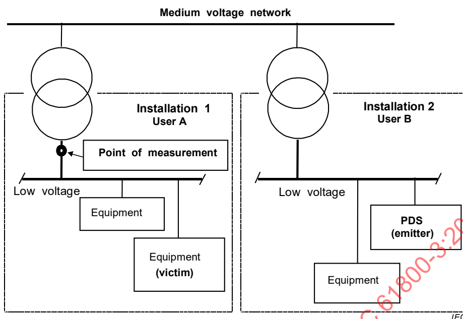
Figure 8 – Propagation of disturbances
