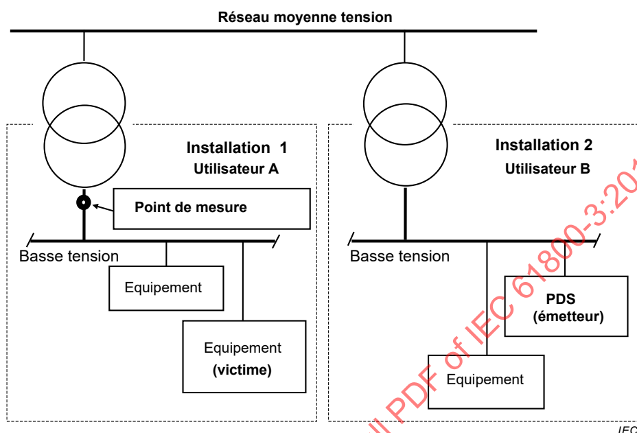
Figure 8 – Propagation des perturbations
