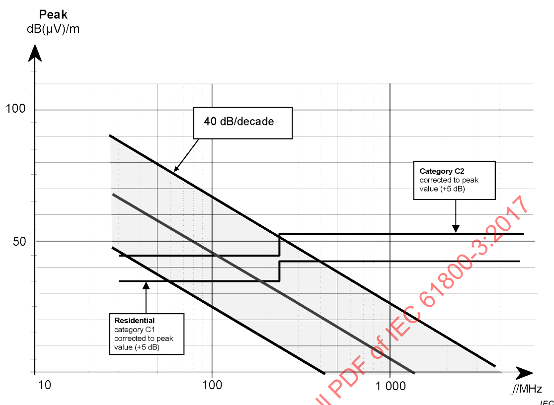
Figure D.2 – Expected radiated emission of PDS up to rated voltage 400 V Peak values normalised at 10 m
