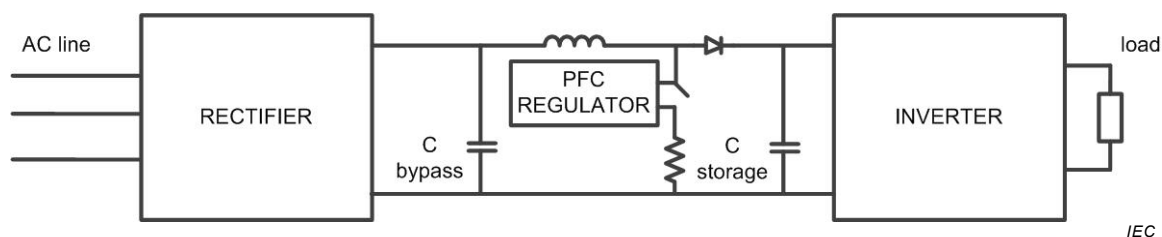
Figure C.7 – Boost mode converter
