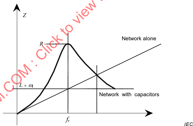
Figure C.3 – Impedance versus frequency of the simplified network
