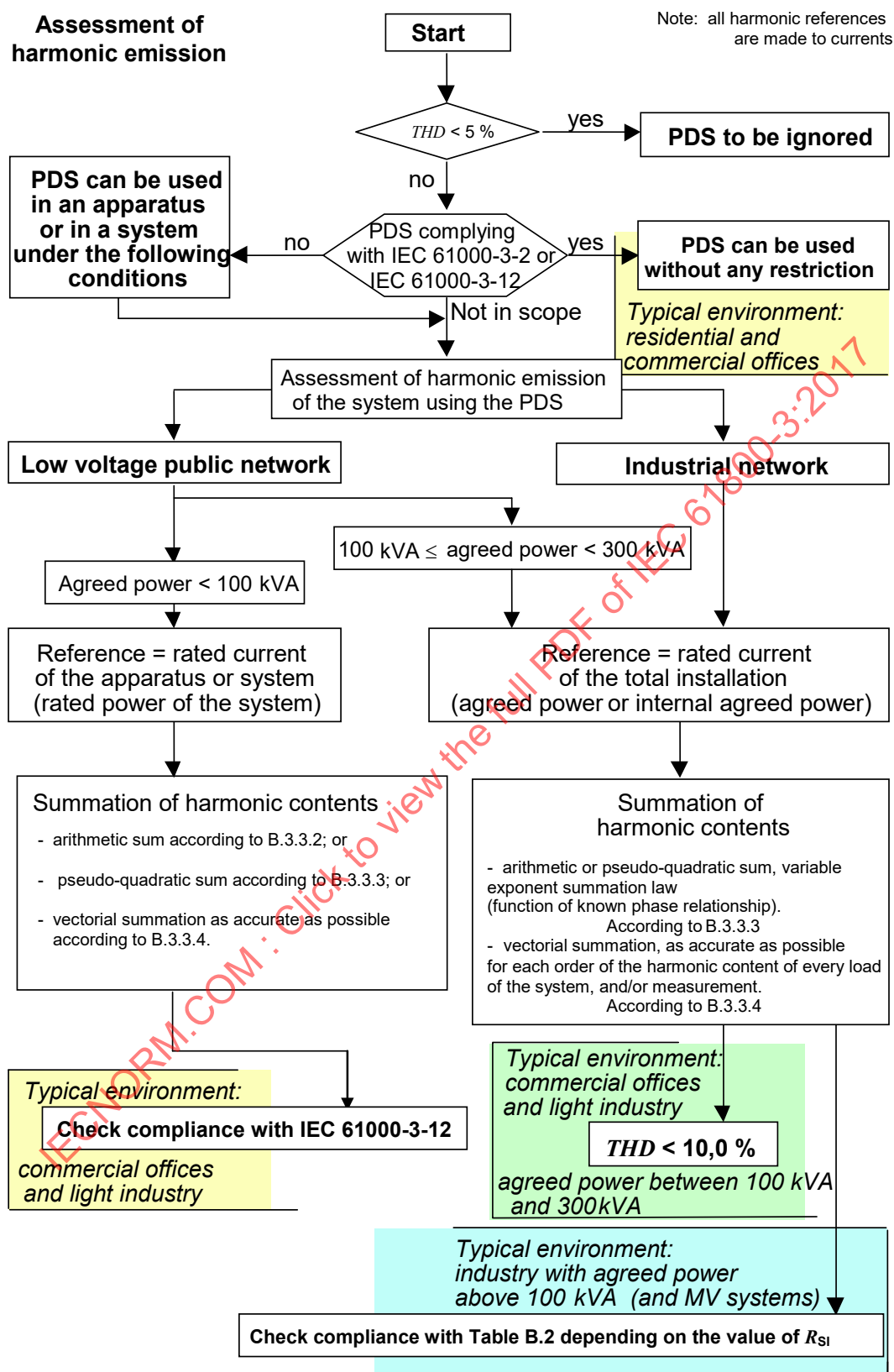
Figure B.8 – Assessment of harmonic emission where PDS is used (apparatus, systems or installations)
