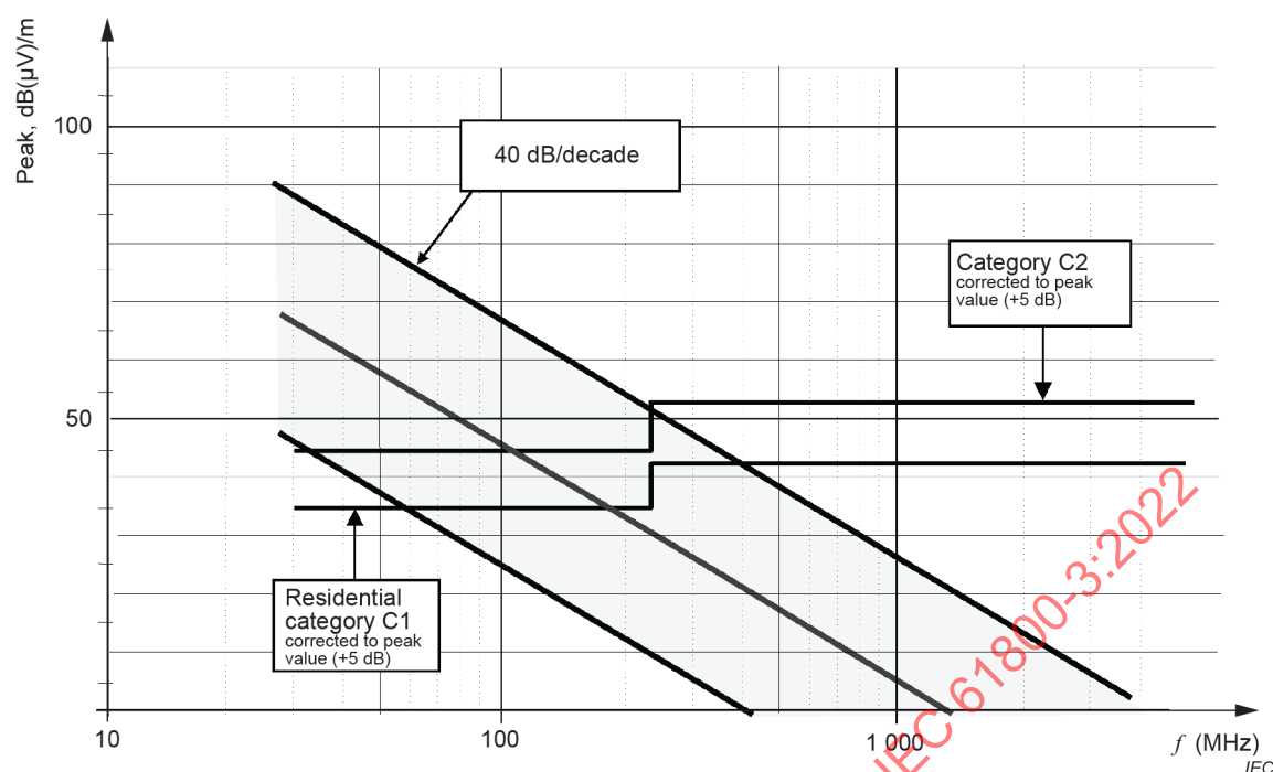
Figure D.2 – Expected radiated emission of EUT up to rated voltage 400 V – Peak values normalised at 10 m
