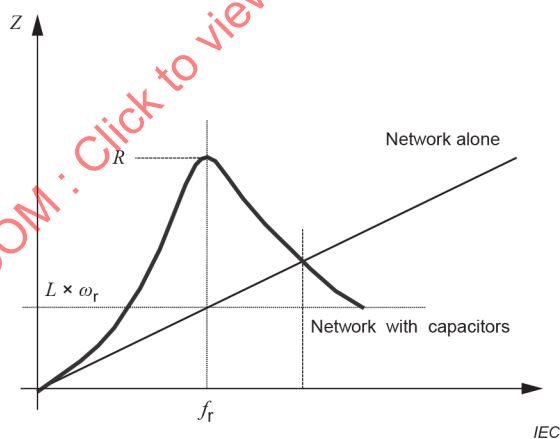
Figure C.3 – Impedance versus frequency of the simplified network
