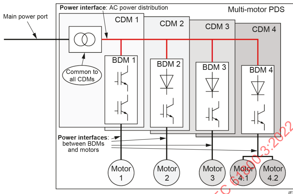
Figure 6 – Power interfaces with common input transformer
