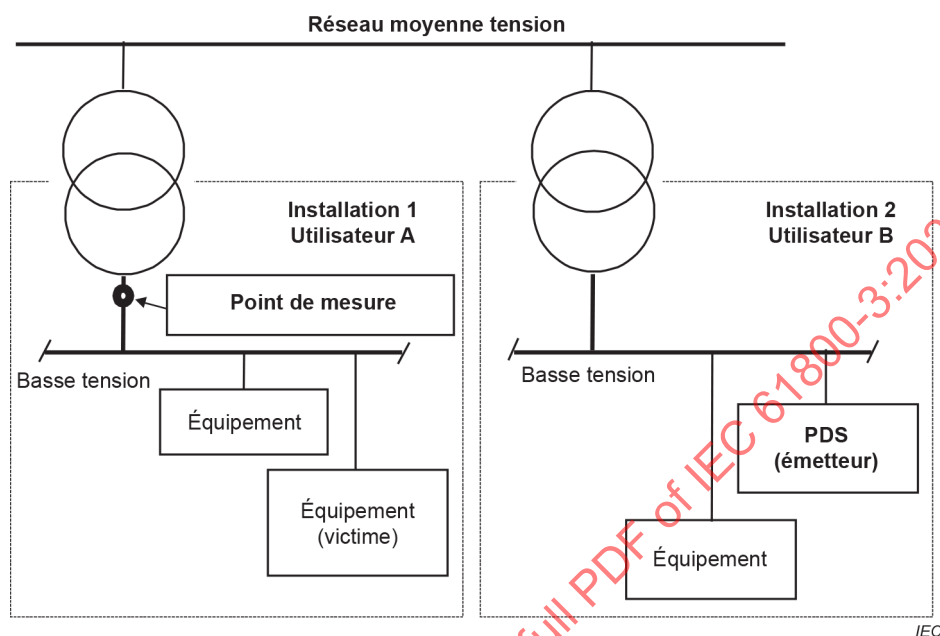
Figure 11 – Propagation des perturbations
