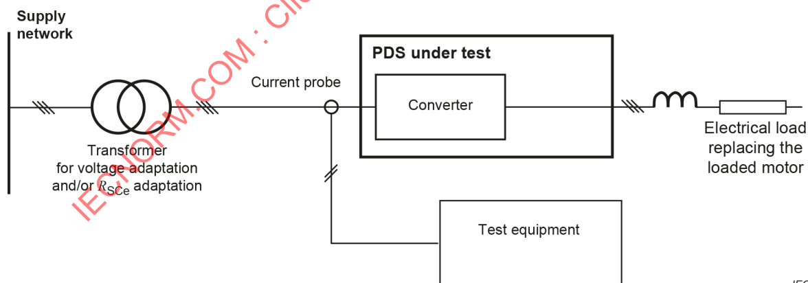
Figure B.6 – Test set-up with electrical load replacing the loaded motor
