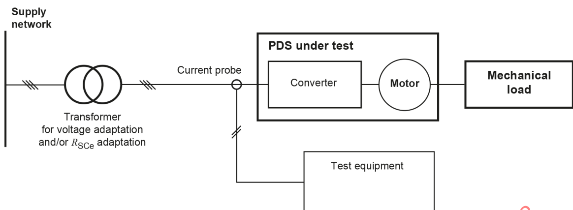
Figure B.5 – Test set-up with mechanical load
