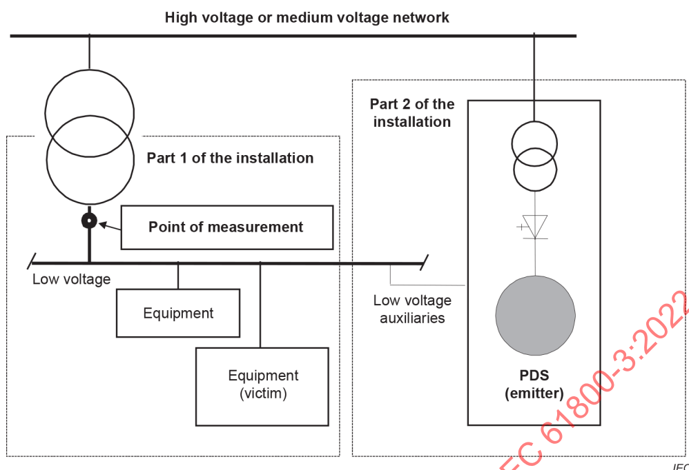
Figure 12 – Propagation of disturbances in installation with an EUT rated > 1 000 V
