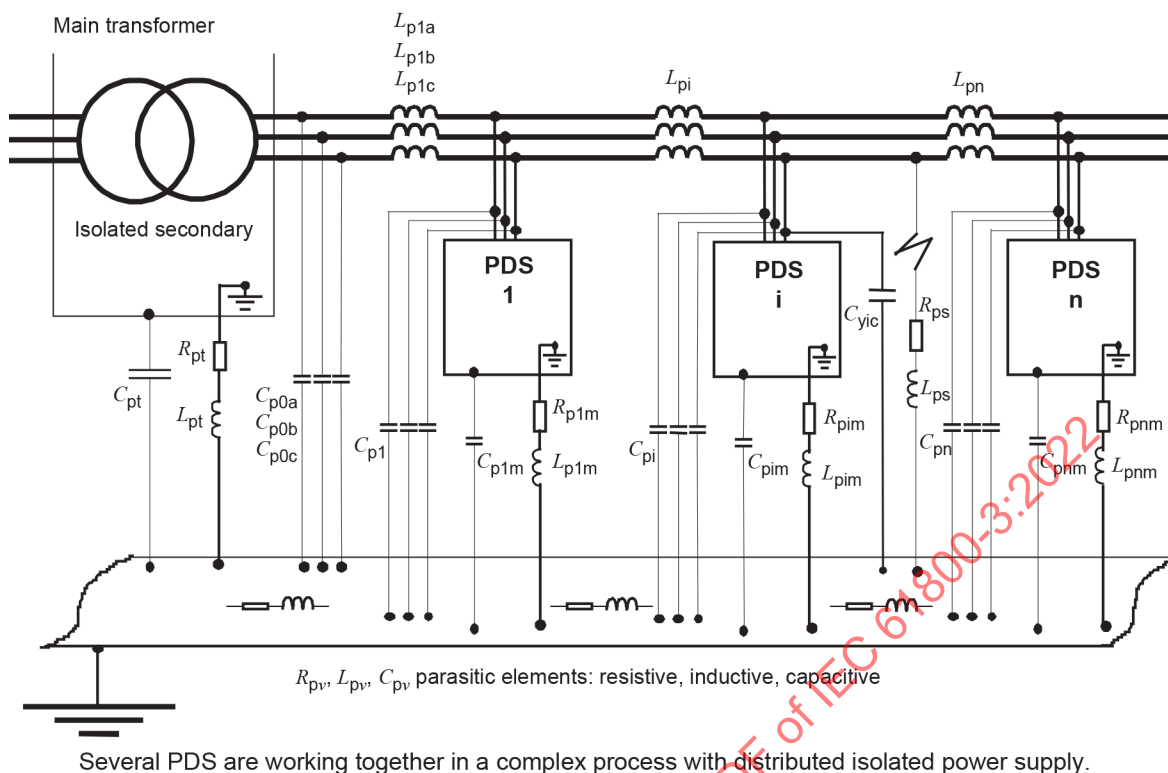
Figure D.3 – Safety and filtering
