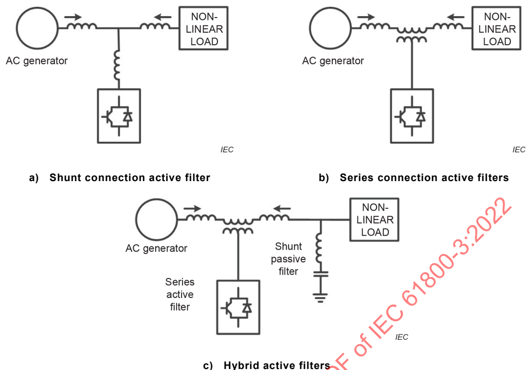
Figure C.6 – VSI PWM active filter topologies
