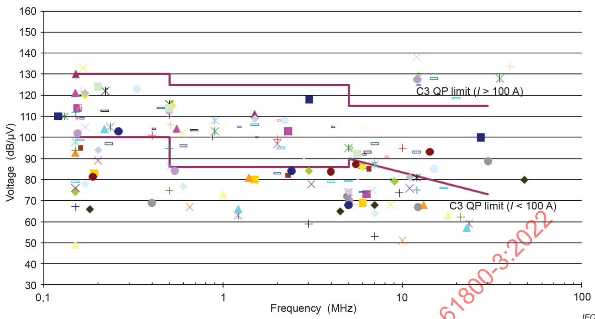
Figure D.1 – Conducted emission of various unfiltered EUTs
