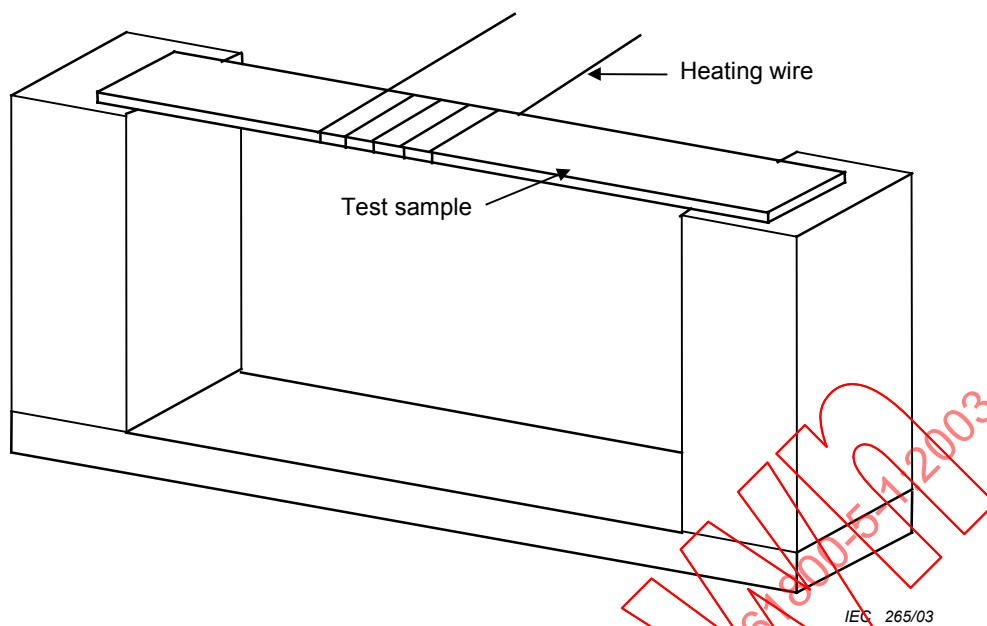
Figure 8 – Test fixture for hot-wire ignition test
