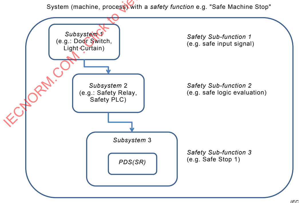
Figure 2 – Safety function consisting of safety sub-functions
