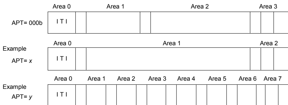
Figure 26 – Division of a track prescribed by APT
