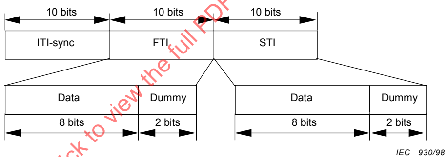
Figure 34 – Structure of a TI-sync block
