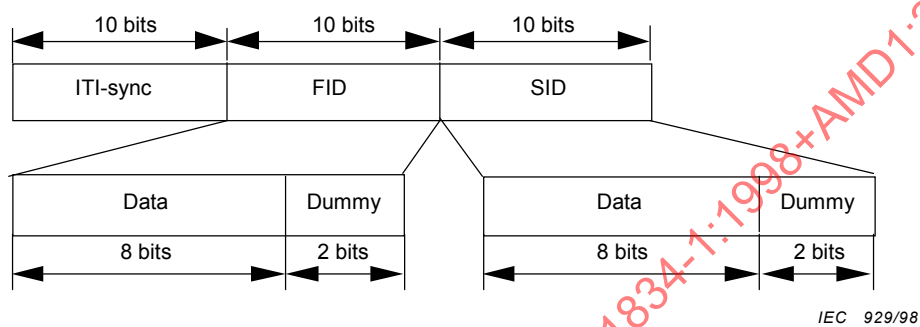
Figure 33 – Structure of a start-sync block
