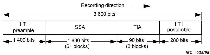
Figure 32 – Structure of ITI sector
