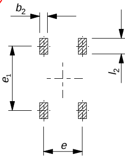
Terminal configuration
