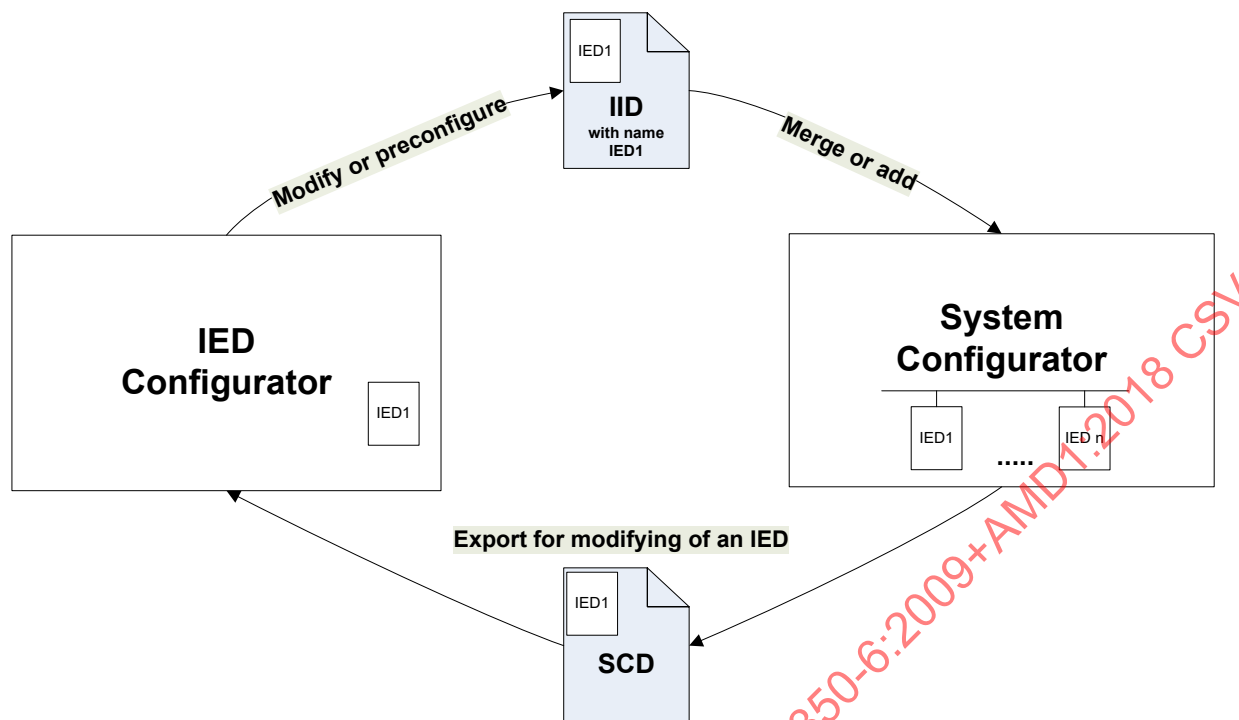
Figure 3 – IED instance description to System Configurator
