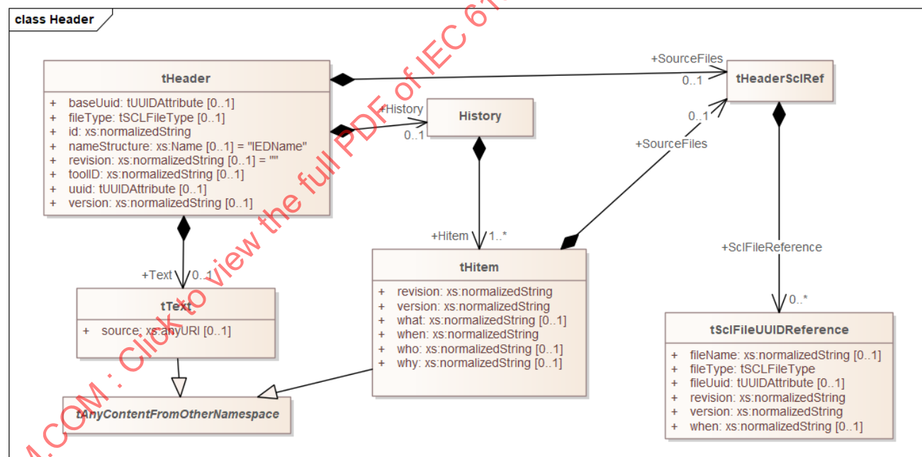
Figure 14 – UML diagram of Header section
