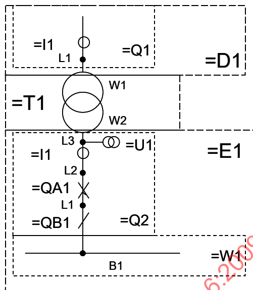
Figure 17 – Substation section example
