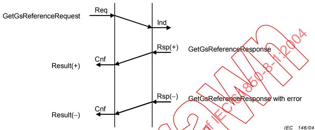
Figure 11 – GetGsReference service primitives
