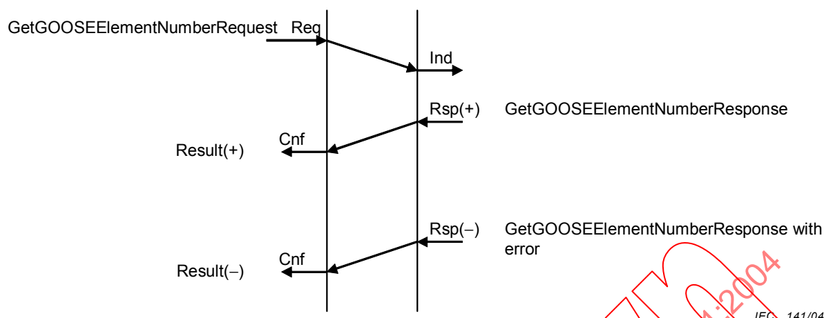
Figure 6 – GetGOOSEElementNumber service primitives
