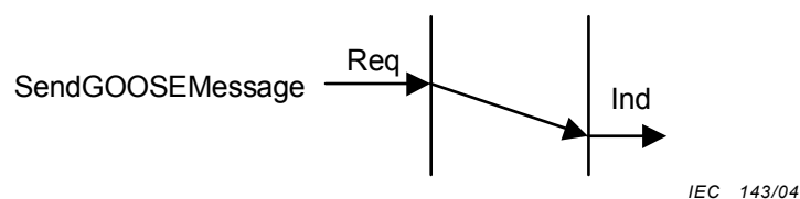
Figure 8 – SendGooseMessage message service primitives
