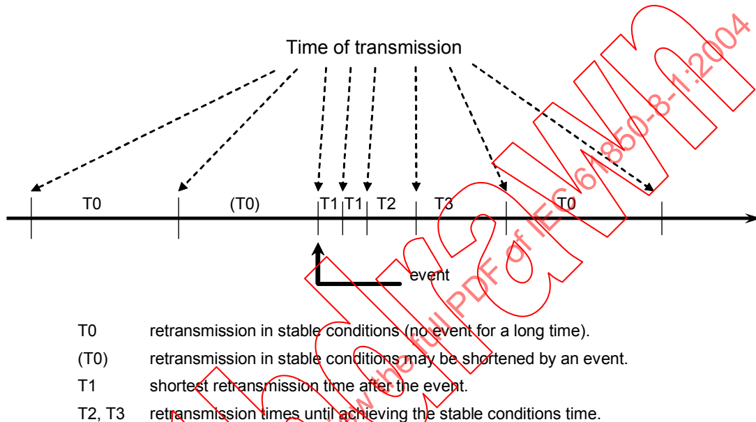
Figure 7 – Transmission time for events
