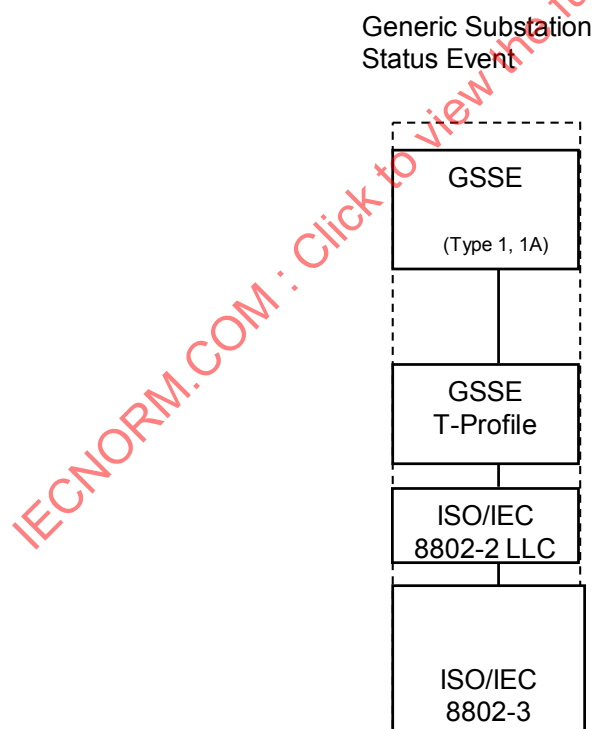
Figure H.1 – Overview of functionality and profiles
