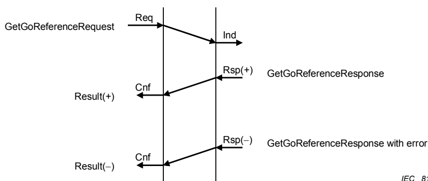
Figure 6 – GetGoReference service primitives
