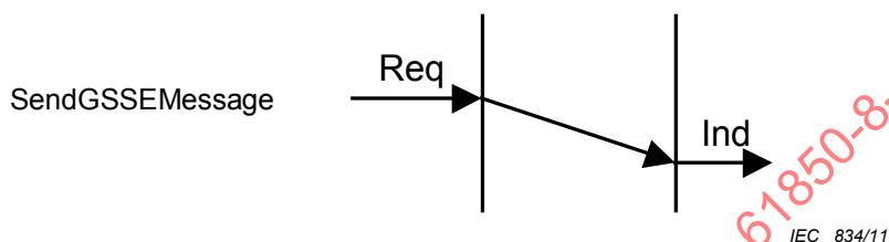
Figure H.4 – GSSE service primitives
