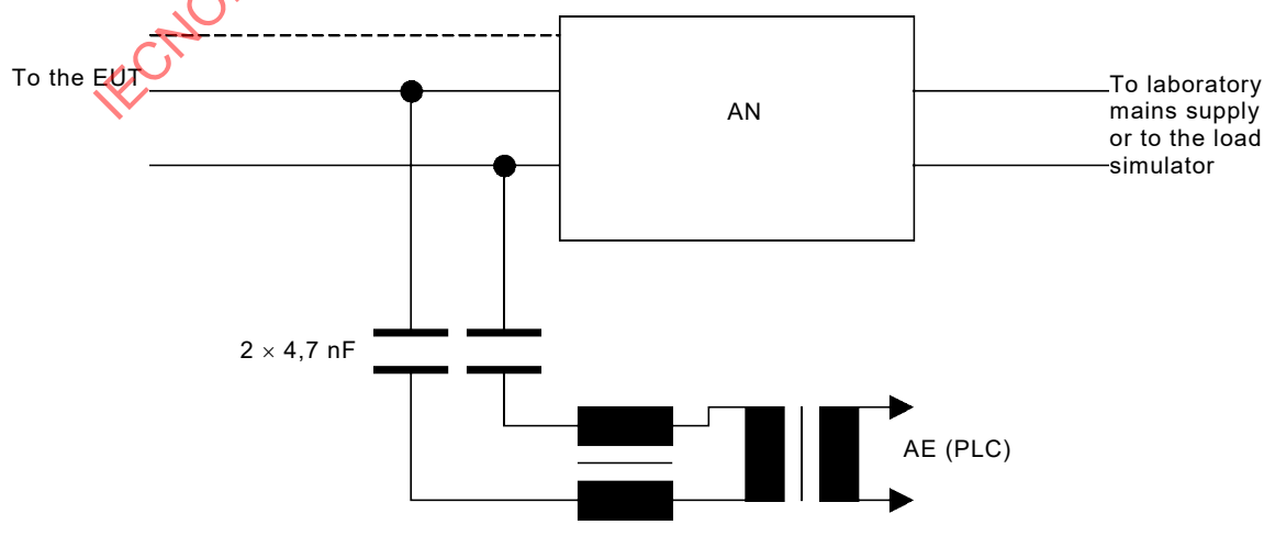
Figure C.3 – Example of a circuit for immunity tests of PLC on AC or DC power lines
