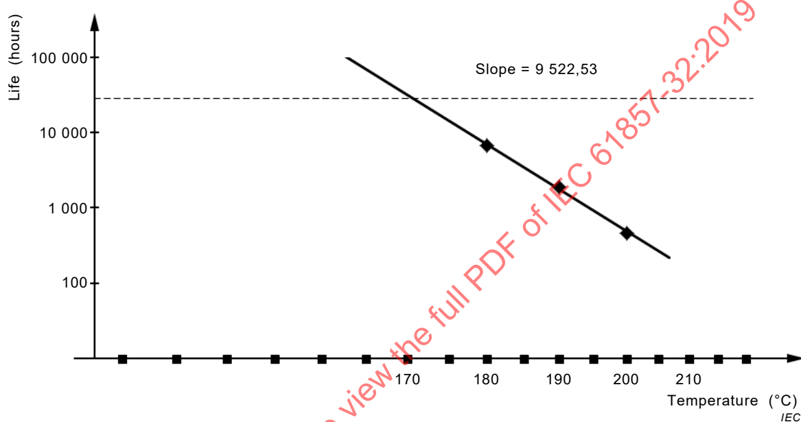
Figure D.1 – Baseline candidate data with the known thermal index of 161 °C when the time coordinate from the reference is 45 200 hours
