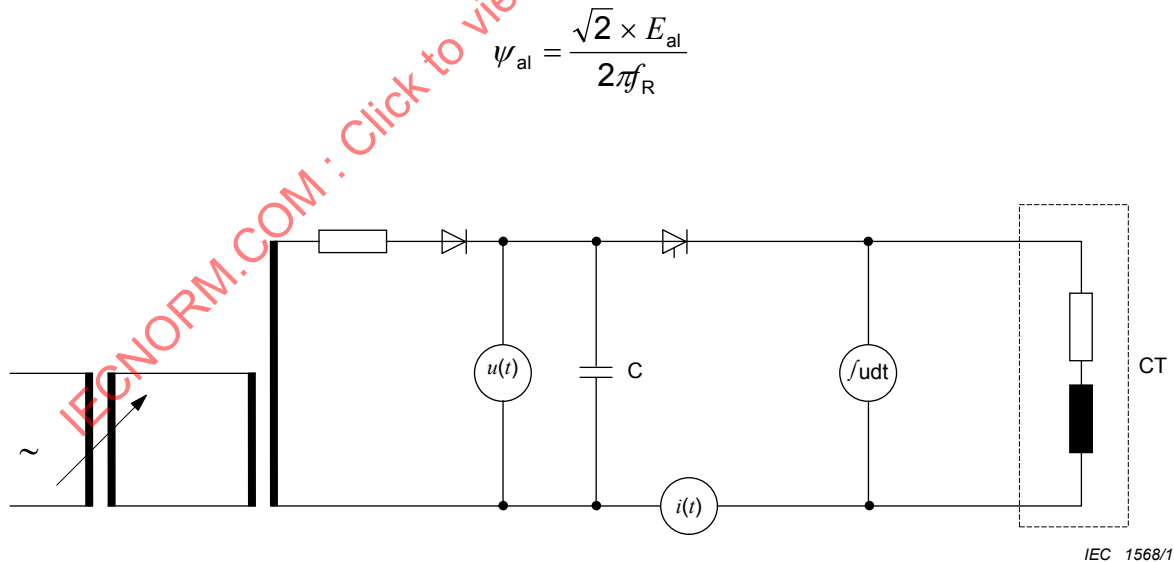
Figure 2B.13 – Circuit for capacitor discharge method
