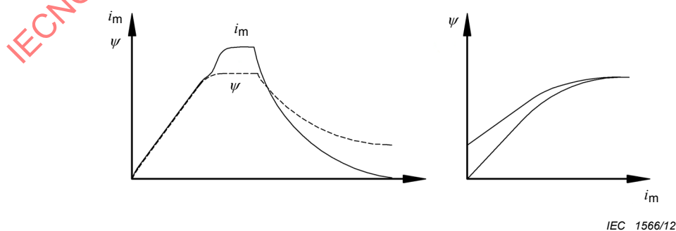
Figure 2B.11 – Time-amplitude and flux-current diagrams
