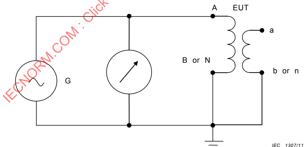
Figure 314 – Differential mode (induced) test voltage application – Primary excitation
