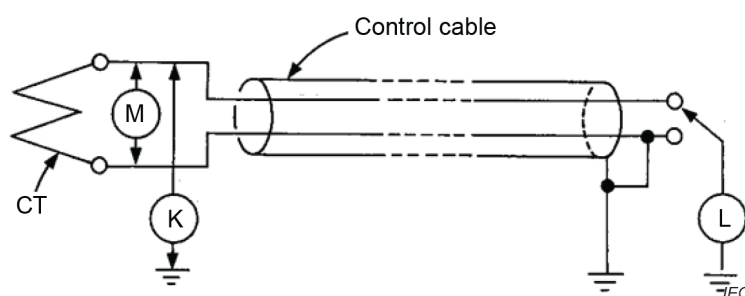
Figure 13B.8 – CT secondary circuit configuration for the 500 kV GIS
