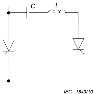
Figure A.1b – Commutating circuit example
