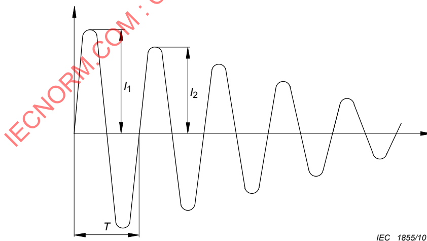
Figure C.3 – Discharge current wave shape
