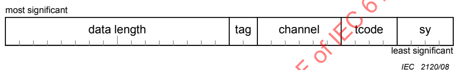
Figure 4 – Isochronous packet header
