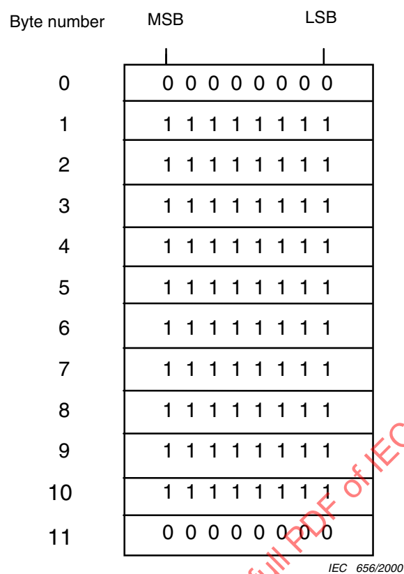
Figure 23 – Layout of the sync field
