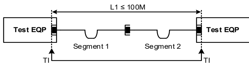
Figure O.4 – Two Segment, three Connection E2E link
