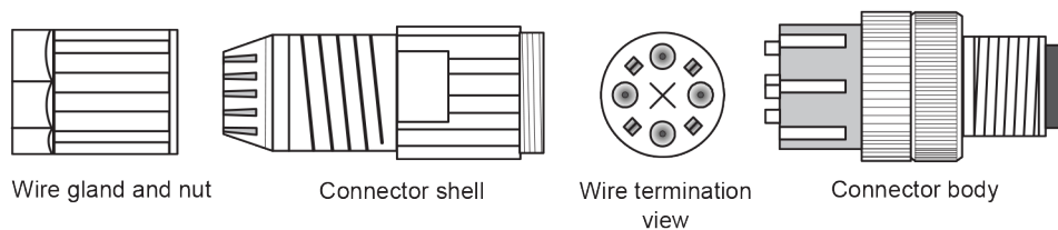
Figure I.7 – Connector components
