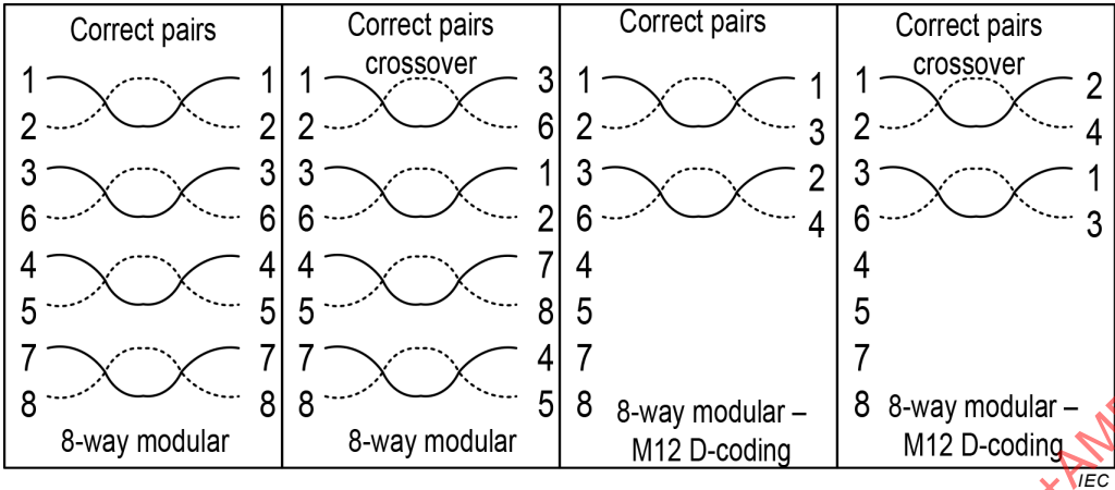
Figure 43 – Pin and pair grouping assignments for two eight position IEC 60603-7 subparts and four position IEC 60603-7 series to IEC 61076-2-101 connectors
