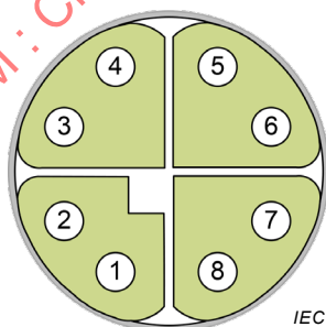
Female contacts
