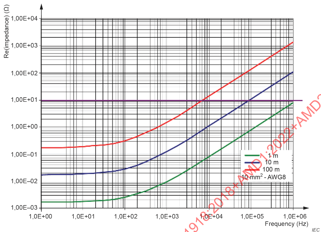
Figure 16 – Impedance of the earthing conductors and equalisation conductors versus noise frequency
