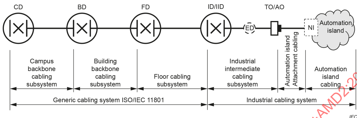
Figure 3 – Automation island cabling attached to elements of generic cabling
