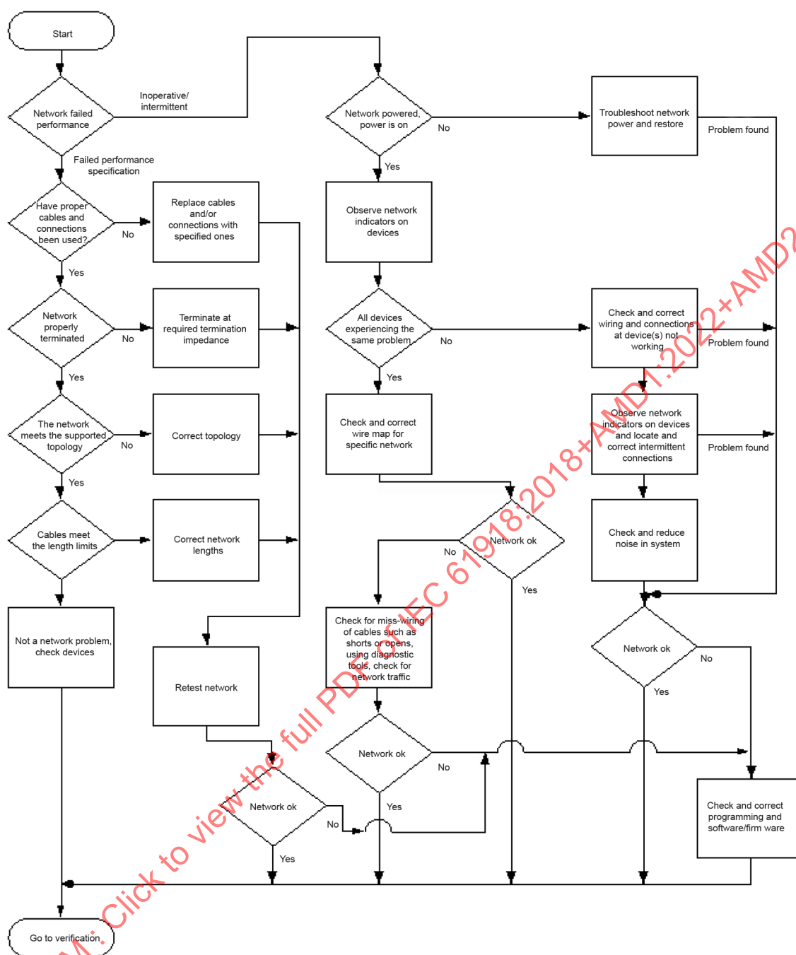
Figure 51 – Troubleshooting procedure
