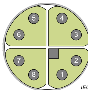
Male contacts
