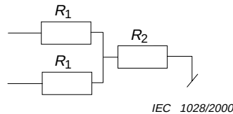
Figure 1 – Resistor load
