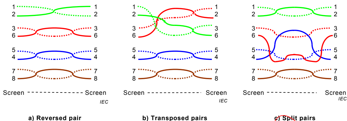
Figure 18 – Incorrect pairing
