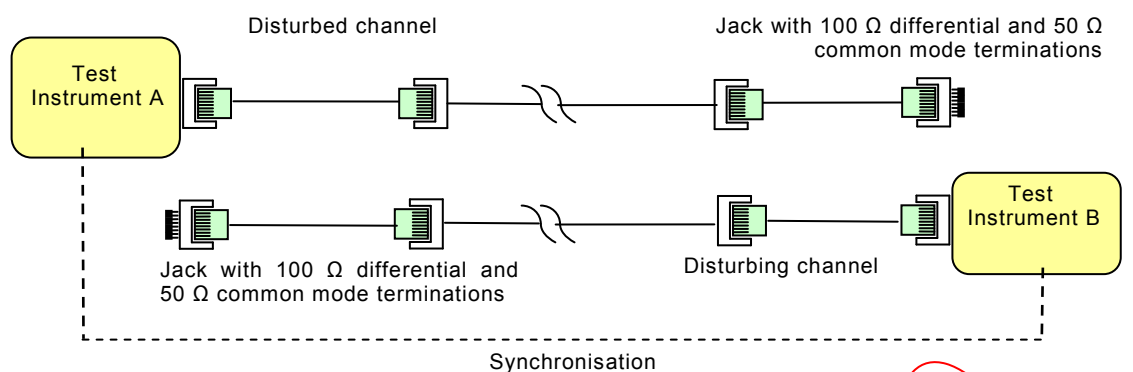
Figure 20 – AFEXT loss measurement test configuration
