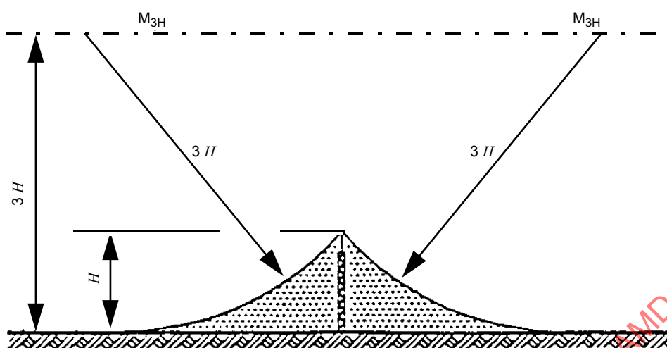
Figure E.3 – Single lightning rod
