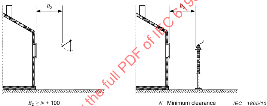
Figure 4b – Outer wall with screened windows
