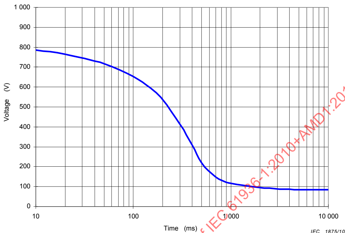
Figure 12 – Permissible touch voltage U_{Tp}
