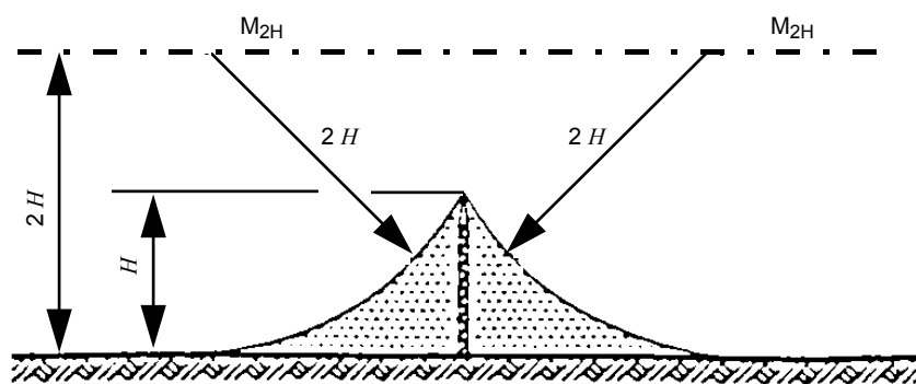
Figure E.1 – Single shield wire
