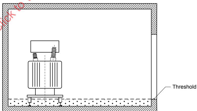
Figure 10 – Sump with integrated common catchment tank
