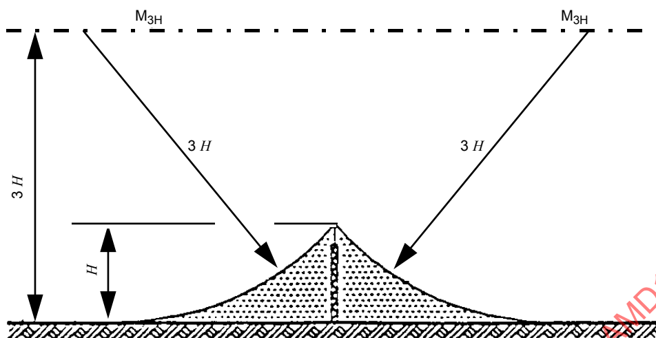
Figure E.3 – Single lightning rod
