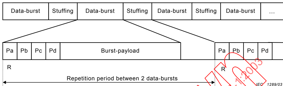
Figure 2 – Data-burst format
