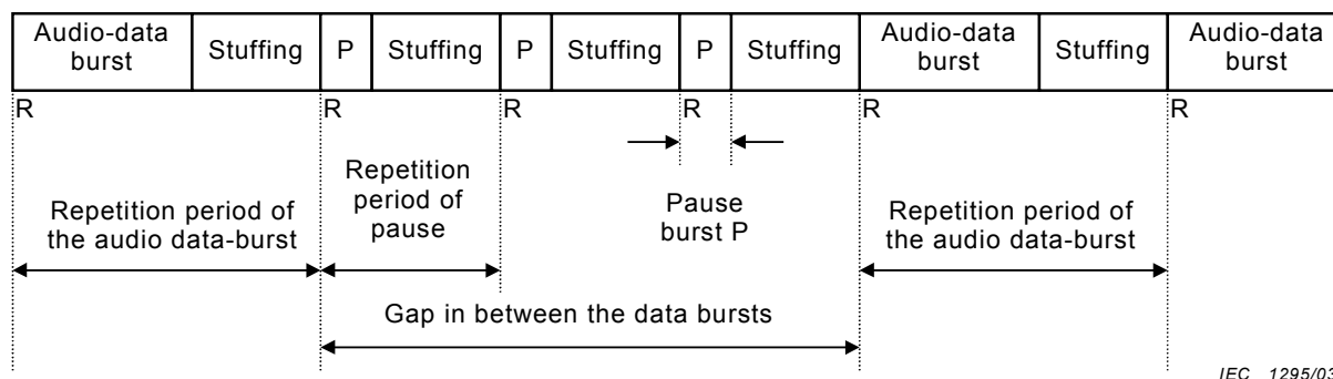
Figure 8 – Bridging gaps in-between data-bursts with 3 pause data-bursts
