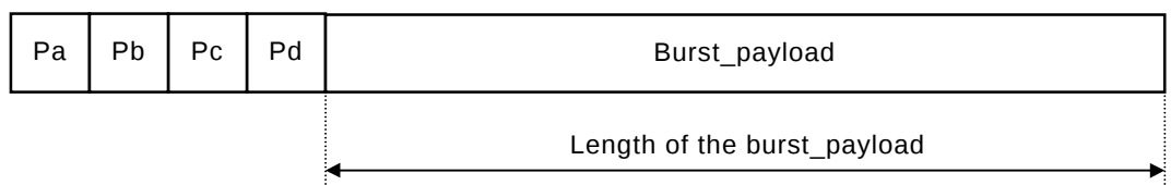
Figure 5 – Length of the burst-payload specified by Pd
