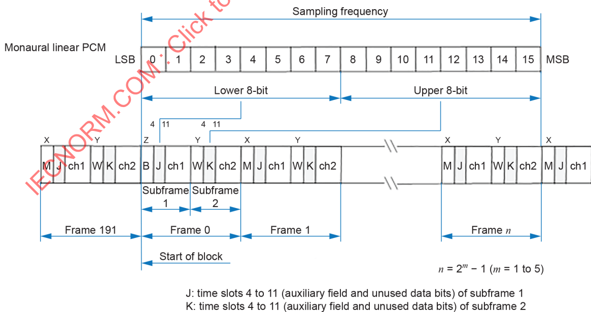
Figure B.1 – Frame and block structure
