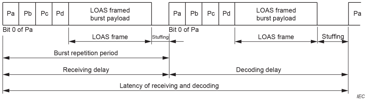
Figure 3 – Latency diagram for burst reception and decoding
