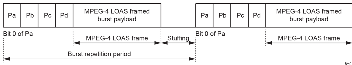
Figure 2 – Data-burst structure
