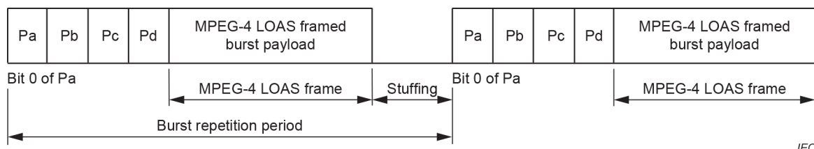
Figure 1 – Data-burst structure
