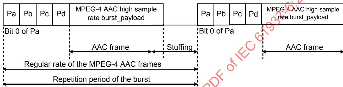
Figure 13 – MPEG-4 AAC double-rate high sampling frequency data-burst
