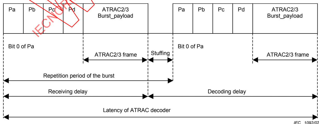
Figure 4 – Latency of ATRAC2/3 decoding
