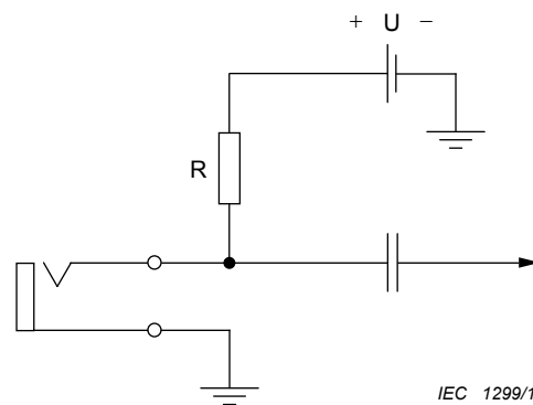
Figure 2 – Example of plug-in power system for a single microphone
