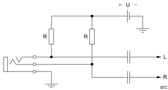
Figure 3 – Example of plug-in power system for a two-channel microphone
