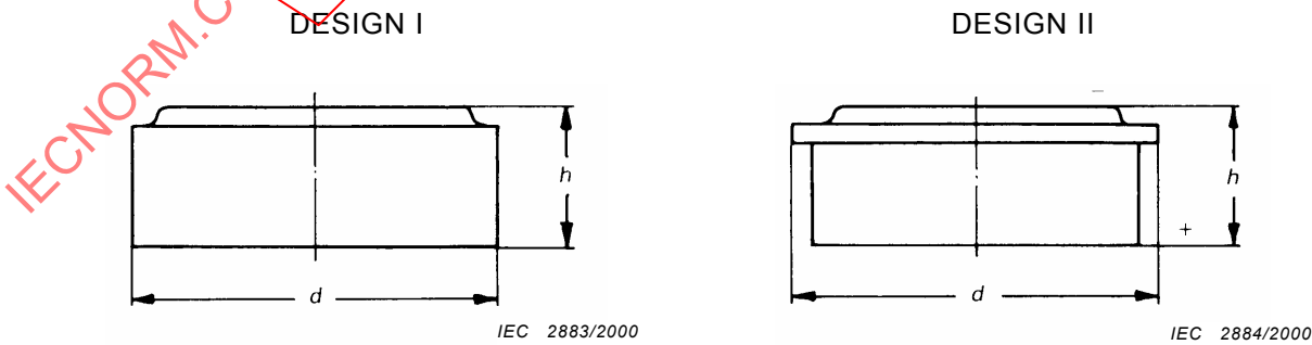
Figure 3 – Button cells
