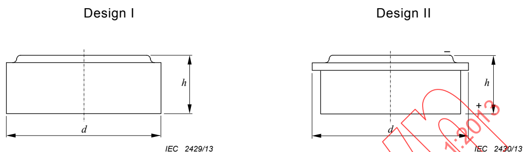
Figure 4 – Button cells
