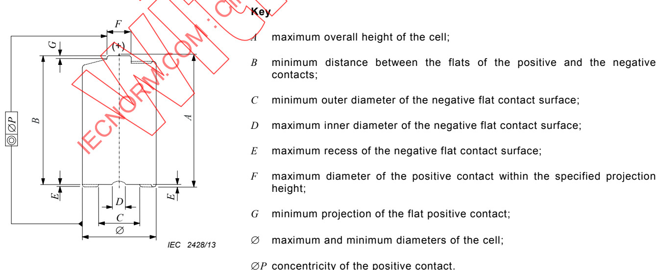
Figure 3 – Jacketed cells dimensionally interchangeable with primary cells
