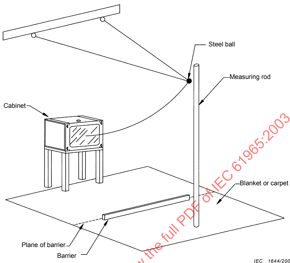
Figure 2 – Example of a ball impact test
