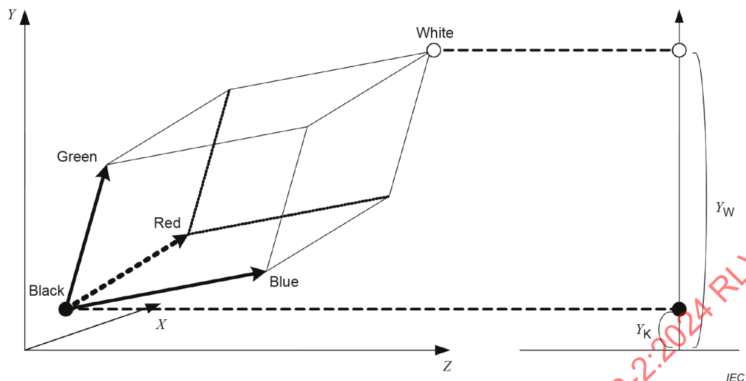
Figure 1 – The colour gamut of additive three primary colours type display for display types comprising three primary additive colours
