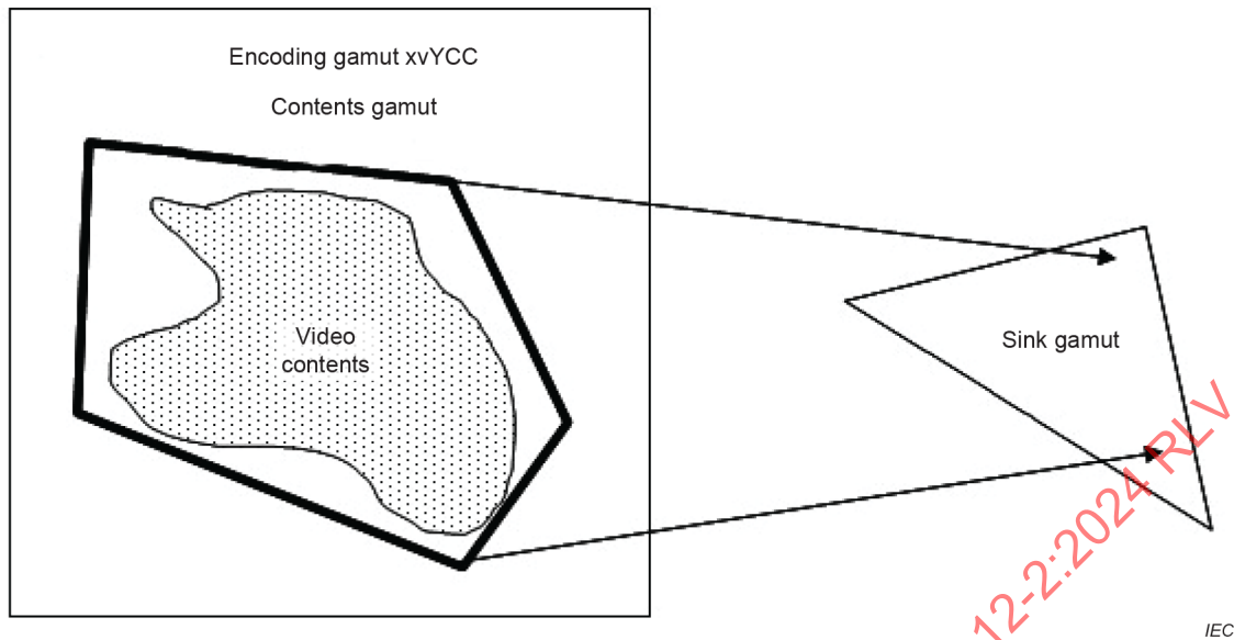
Figure 2 – IEC 61966-12-1 full and medium profiles
