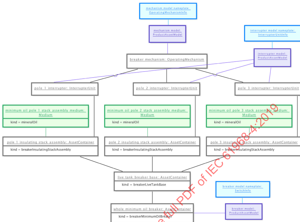
Figure D.14 – Common instance template for minimum oil breaker with 3 insulating stacks on one base, 1 mechanism, single break
