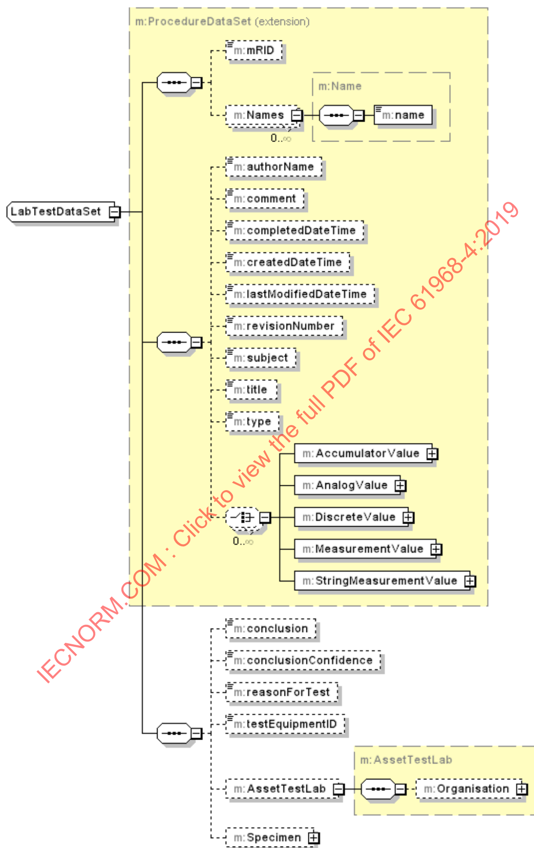
Figure 75 – Message ProcedureDataSets: élément LabTestDataSet
