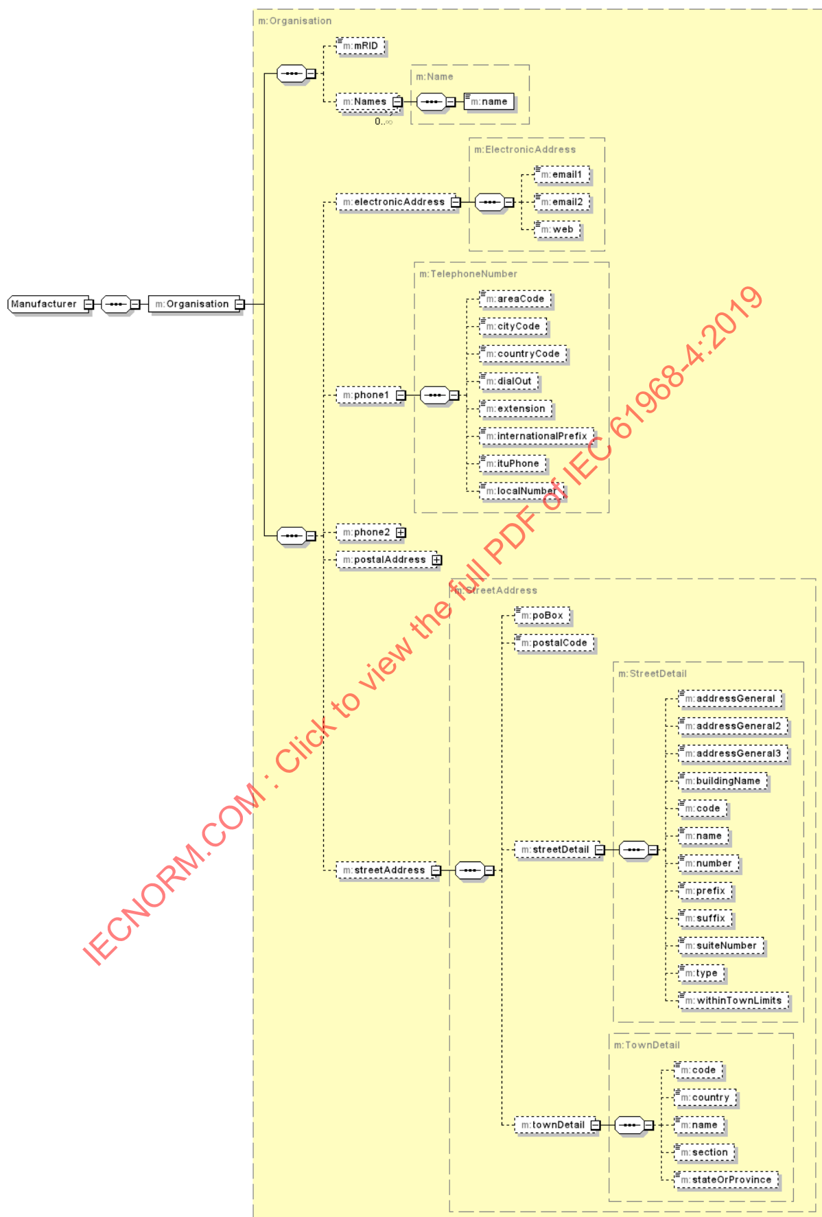
Figure 12 – Message AssetCatalogue: élément Manufacturer
