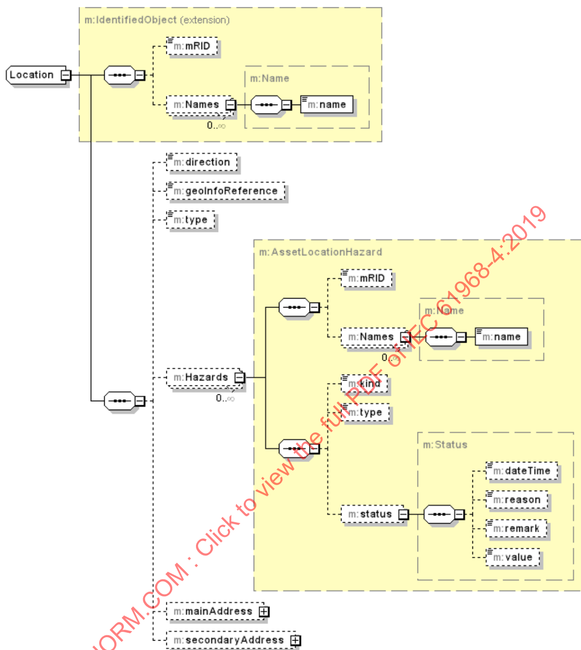
Figure 25 – Message AssetDetail: élément Location
