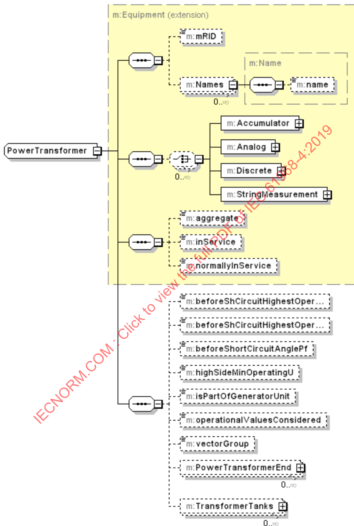
Figure 58 – Message AssetPSRDetails: élément PowerTransformer
