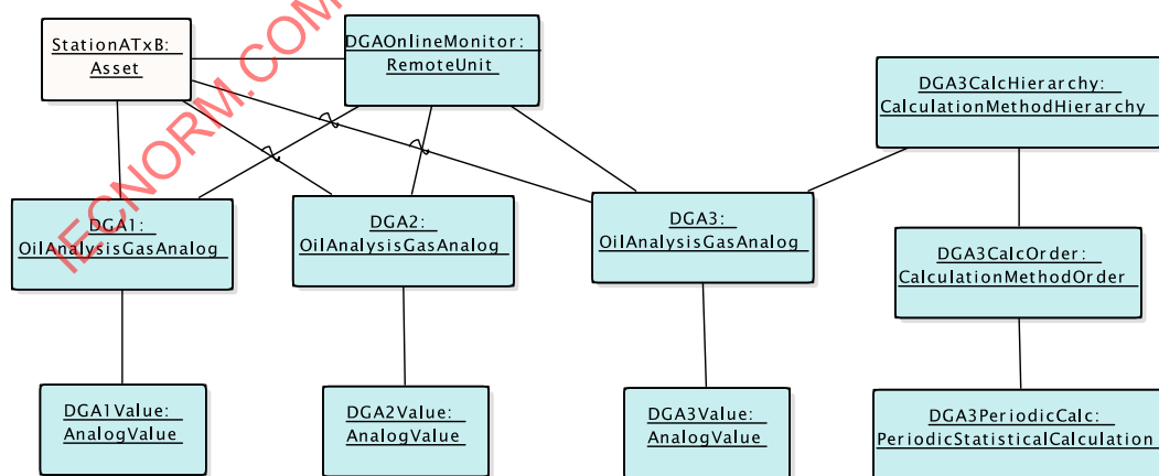
Figure F.3 – Objects instantiated for DGA monitoring
