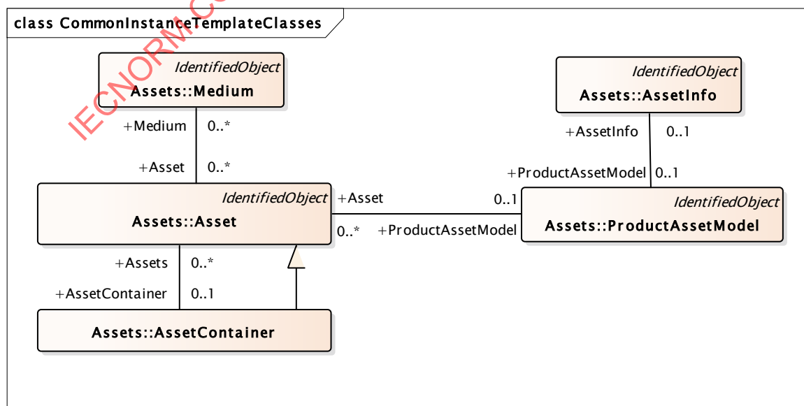
Figure D.2 – Classes utilized in common instance templates
