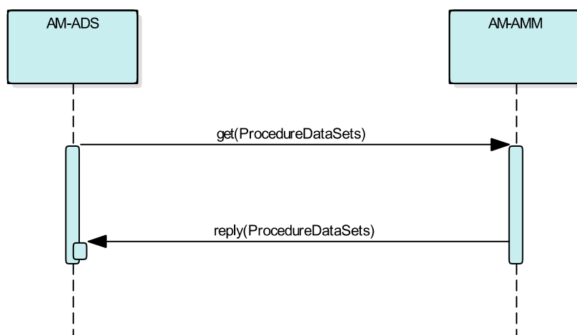
Figure 72 – Échange de messages ProcedureDataSets
