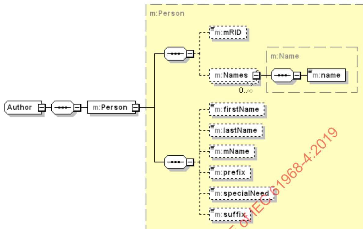
Figure 35 – Message AssetHistory: élément Author
