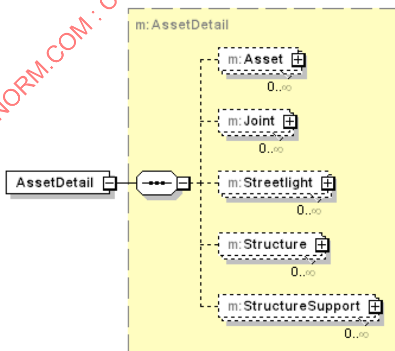
Figure 21 – Format de message AssetDetail
