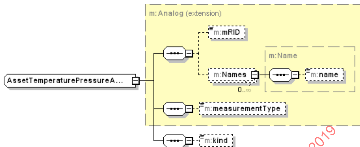
Figure 71 – Format de message Procedures: élément AssetTemperaturePressureAnalog
