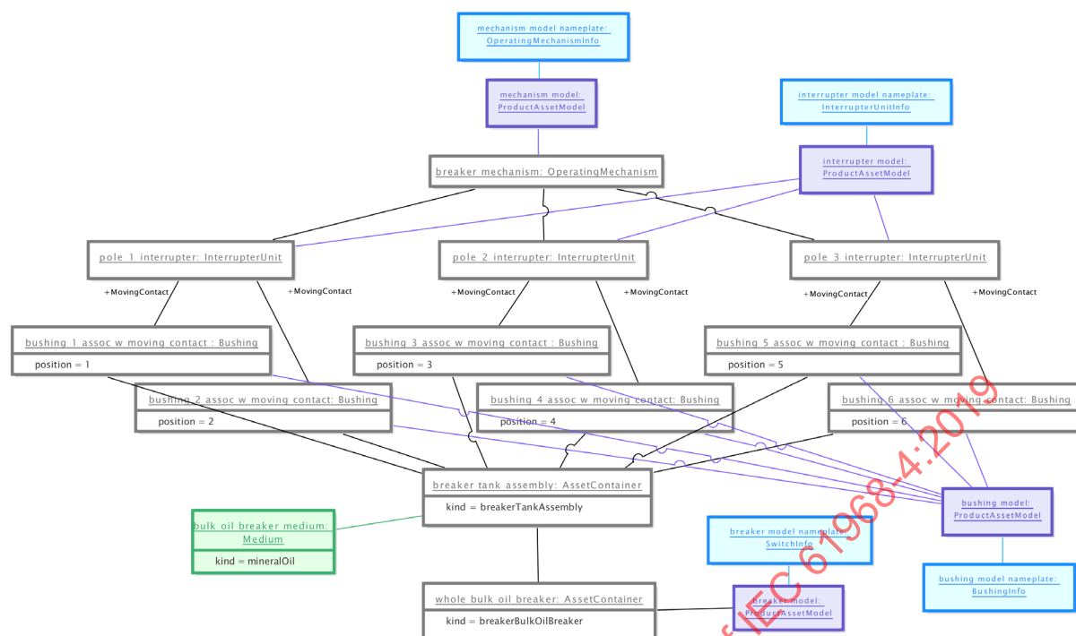
Figure D.11 – Common instance template for bulk oil breaker with 1 tank, 1 mechanism
