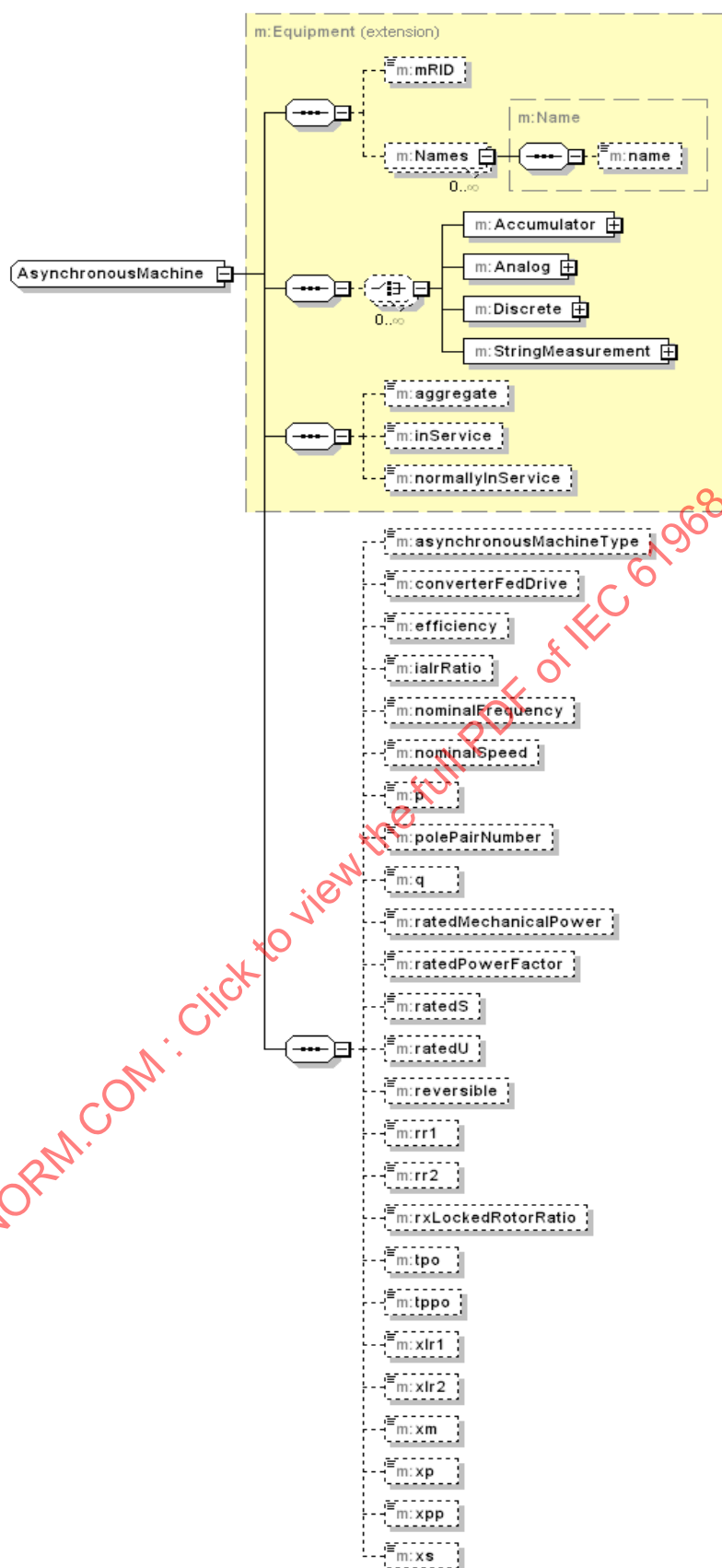
Figure 46 – Message AssetPSRDetails: élément AsynchronousMachine
