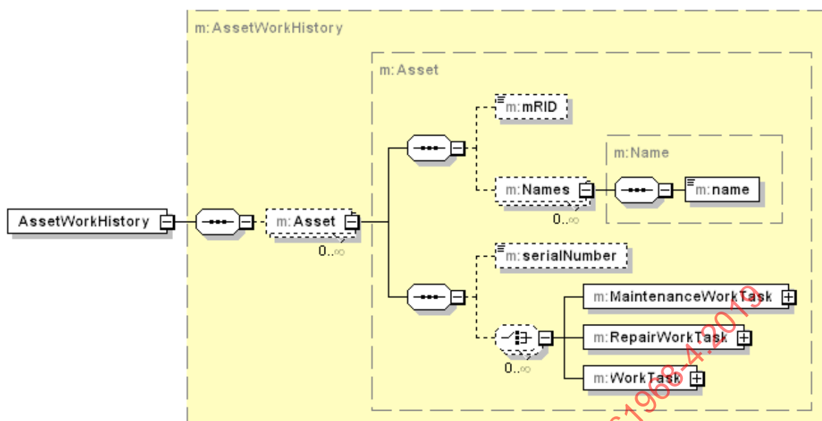
Figure 37 – Format de message AssetWorkHistory
