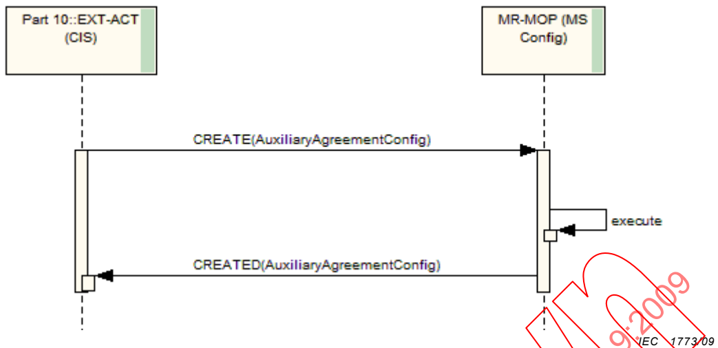
Figure 56 – Message exchange for transferring auxiliary agreement information
