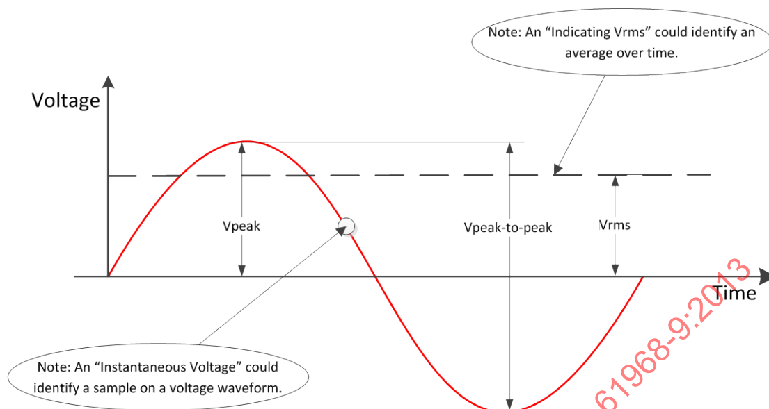
Figure C.3 – Voltage measurements
