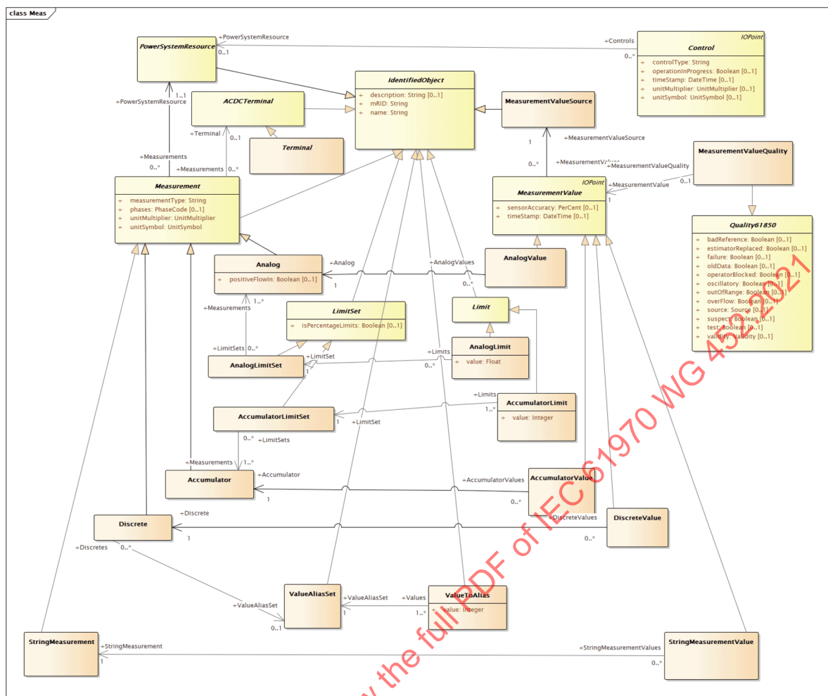
Figure 29 – Class diagram OperationProfile::Meas
