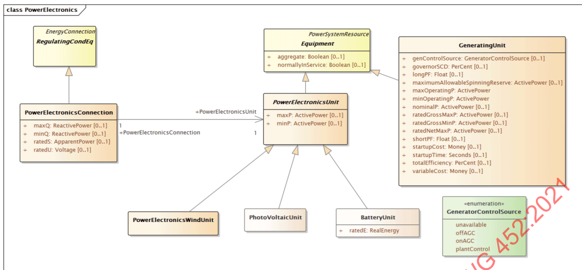
Figure 16 – Class diagram CoreEquipmentProfile::PowerElectronics
