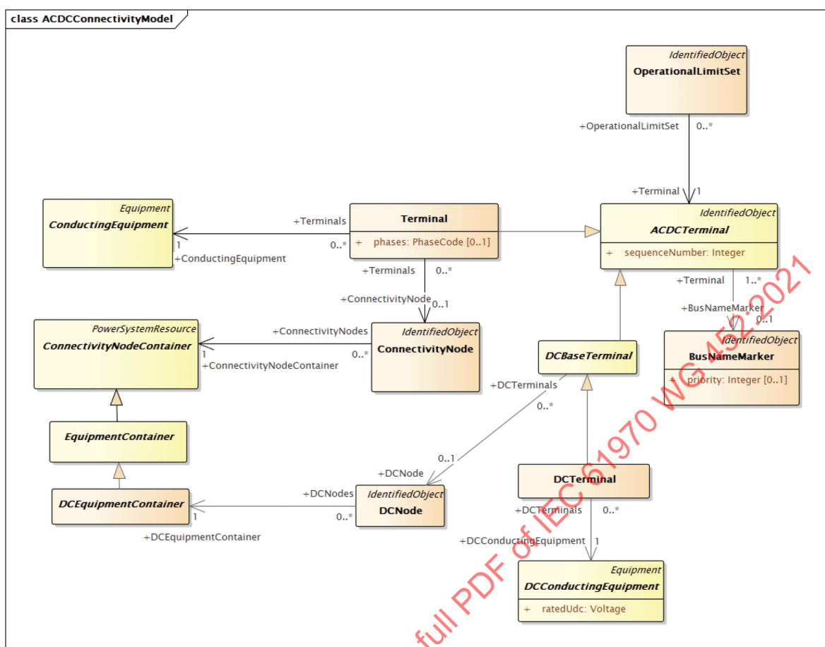
Figure 6 – Class diagram CoreEquipmentProfile::ACDCConnectivityModel
