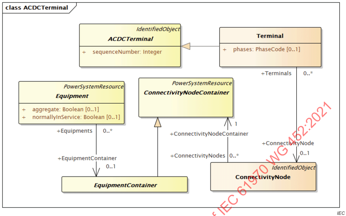
Figure 5 – Class diagram CoreEquipmentProfile::ACDCTerminal
