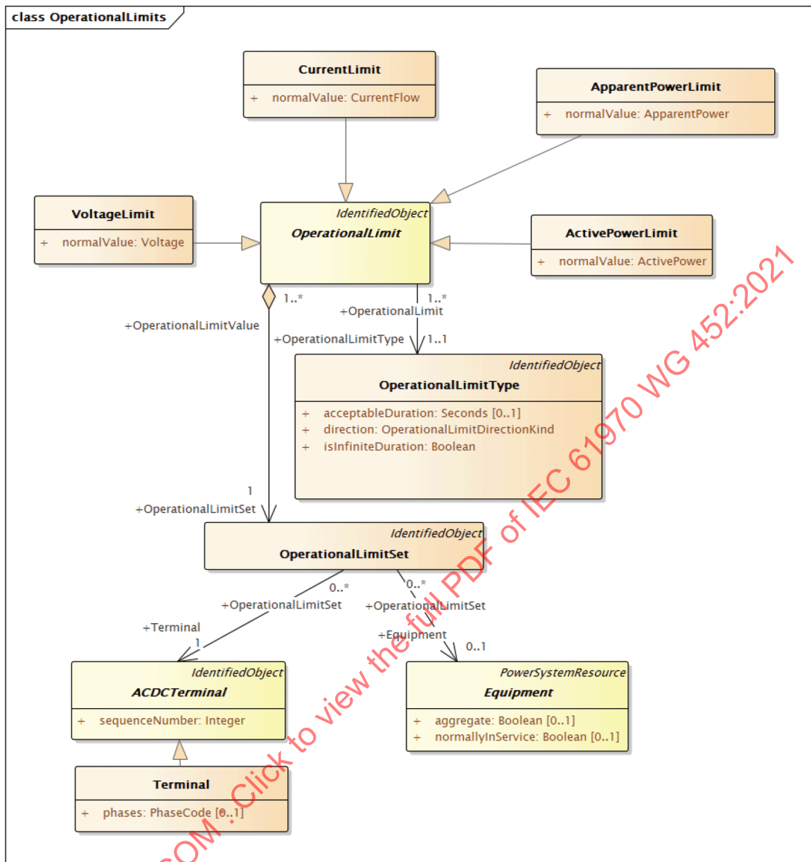
Figure 23 – Class diagram CoreEquipmentProfile::OperationalLimits
