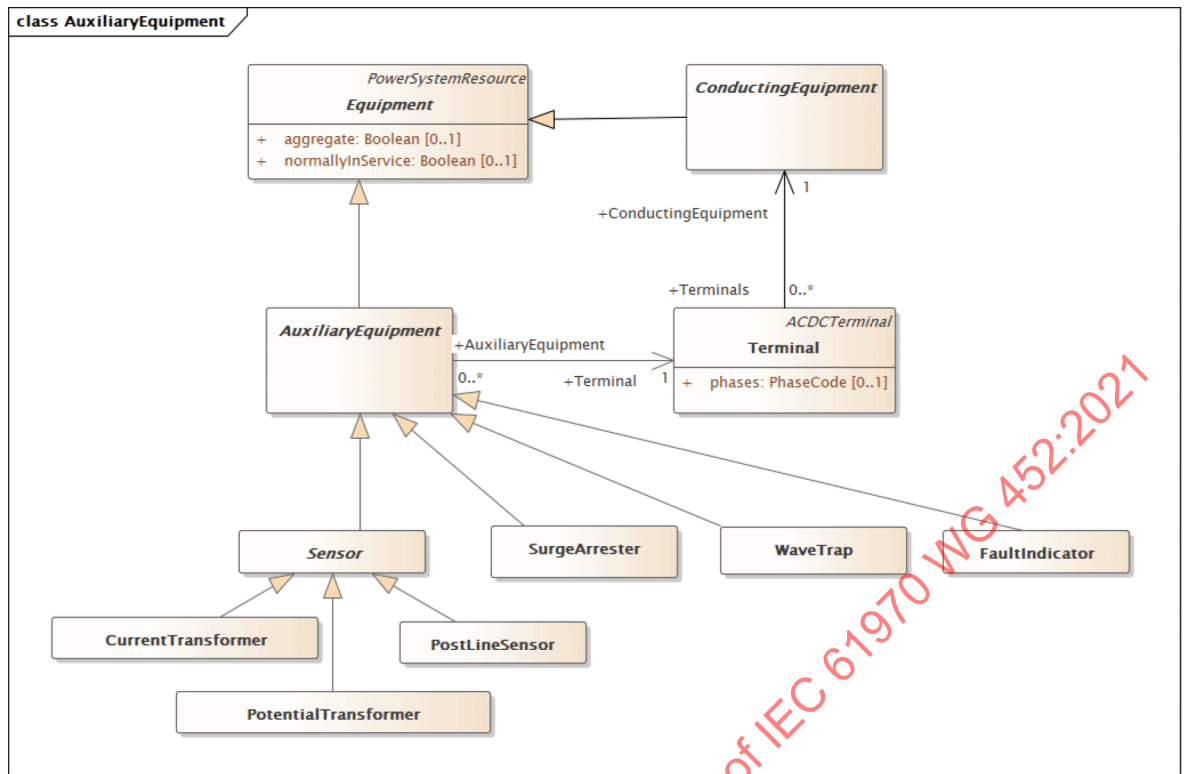
Figure 7 – Class diagram CoreEquipmentProfile::AuxiliaryEquipment
