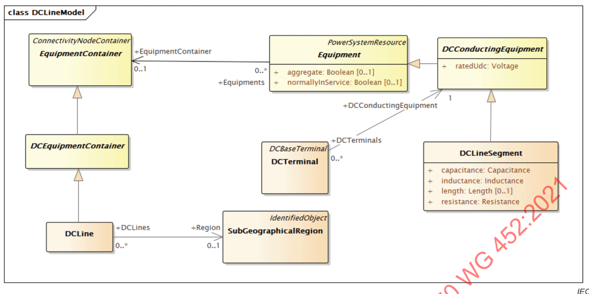
Figure 12 – Class diagram CoreEquipmentProfile::DCLineModel
