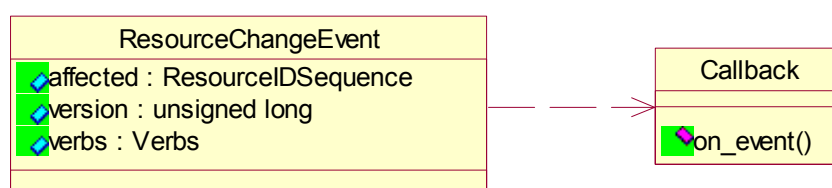
Figure 8 – GDA event model
