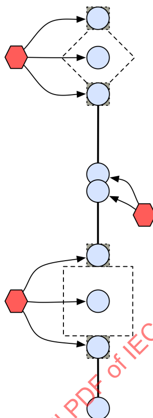
Figure 10 – Disconnect and breaker with glue points
