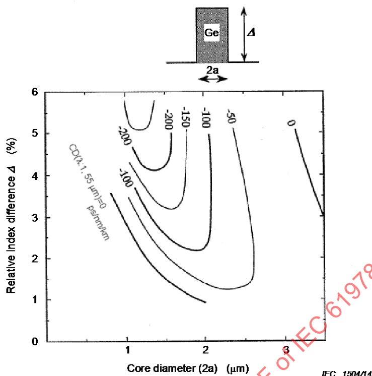
Figure A.2 – Calculated contour for different dispersion at the wavelength of 1,55 \mu\text{m} ( \text{CD}(\lambda:1,55 \mu\text{m}) ) for a step index core fibre
