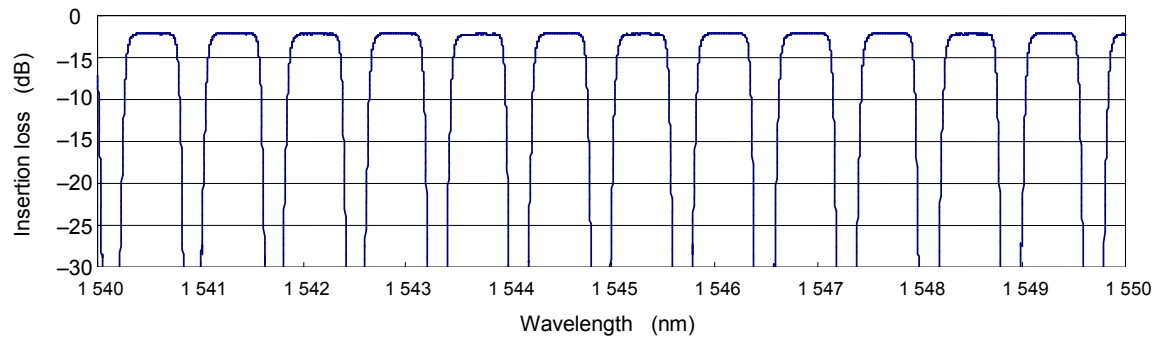
Figure B.2a – Insertion loss including the optical circulator
