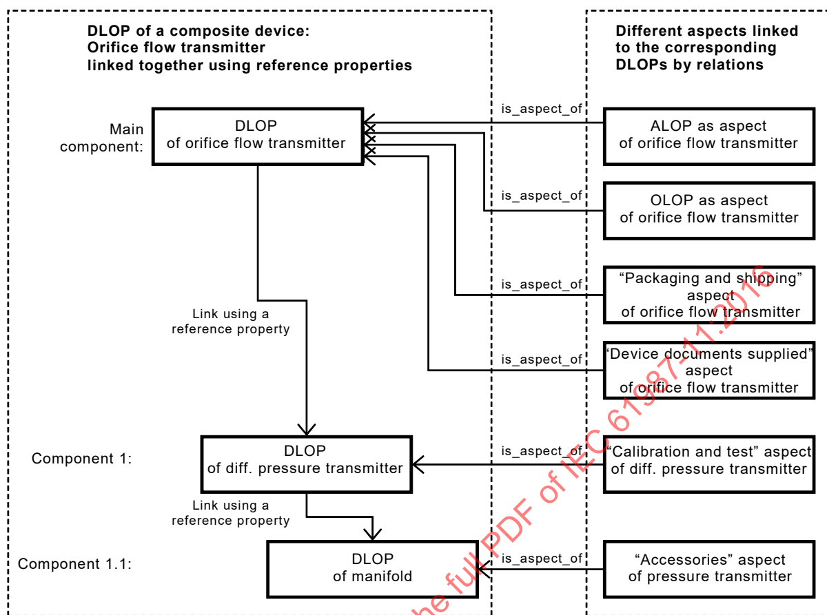
Figure 5 – Example for the structure of an LOP for a composite device showing different aspects related to different sub-components
