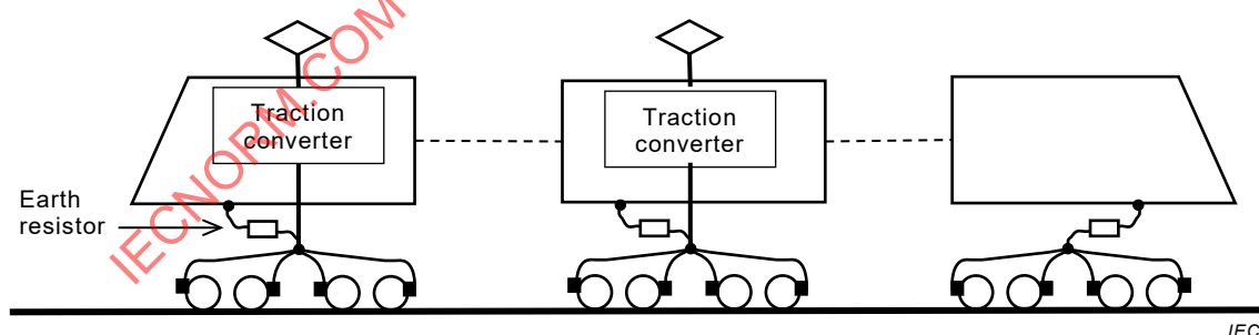
Figure C.2 – Attach earth resistors for long-length EMUs preventing current absorption
