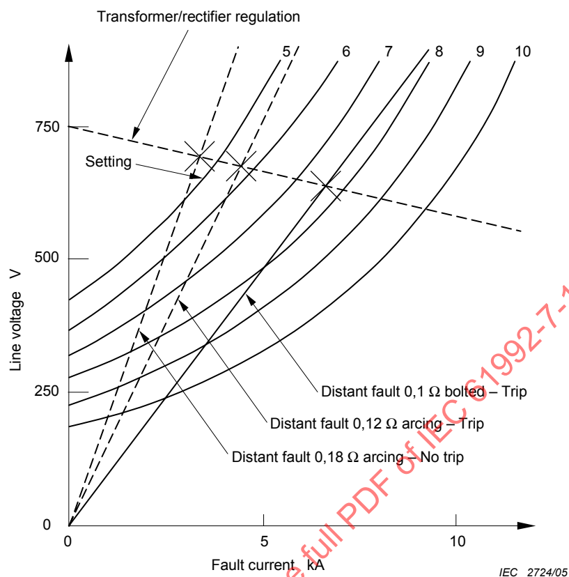
Figure 3 – Typical impedance device (electromagnetic) characteristics and settings
