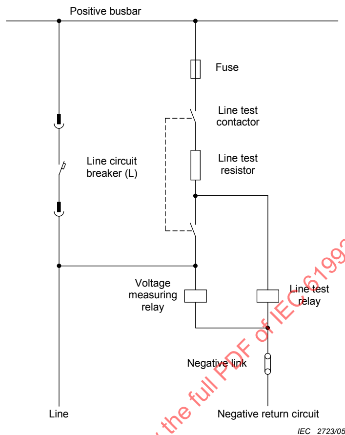
Figure 2 – Basic circuit for line test device
