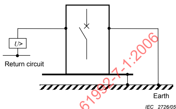
Earthed system without current detection
