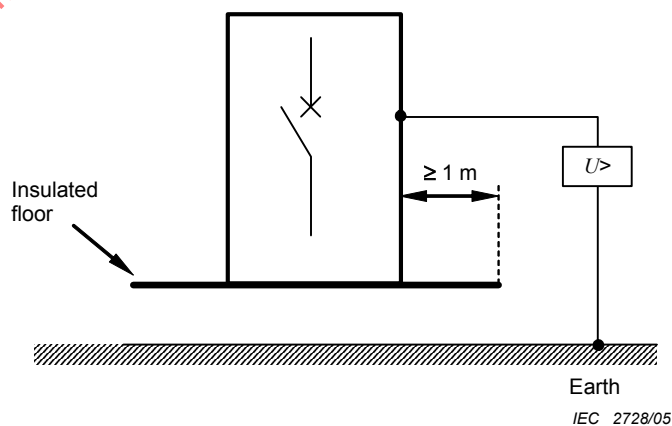
Figure 4c – High impedance system
