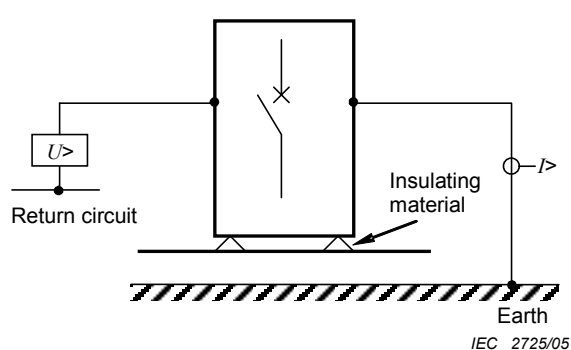
Earthed system with current detection
